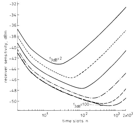
Fig. 10 Receiver sensitivity as a function of n at 50.0 Mbit/s with m = 0.8
