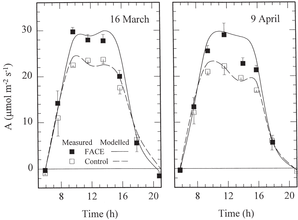
Figure 5. The diurnal course of the mean ( \pm 1 SD) measured leaf CO 2 uptake (symbols) and the predicted leaf CO 2 uptake (lines) for 16 March and 9 April. Predicted rates were calculated from a mechanistic model of photosynthesis in which parameters were set with material from the control plots, using as inputs the record of photon flux, leaf temperature, air saturation deficit (Fig. 1) and ambient CO 2 partial pressure recorded simultaneously with the measurements of A and g s . FACE = elevated CO 2 partial pressure of \approx 55 Pa; control = current ambient CO 2 partial pressure of \approx 37 Pa.
