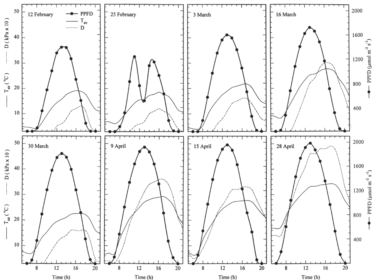
Figure 1. Diurnal courses of air temperature ( T_{\text{air}} ), air saturation deficit ( D ), and photosynthetically active photon flux density (PPFD) at Maricopa, Arizona for 8 d of the 1993 growing season. These data, and the data in the other figures, were fitted with a best-fit non-linear regression (Marquardt–Levenberg algorithm). The actual data as well as the fitted curve are shown to better illustrate the daily progression.
