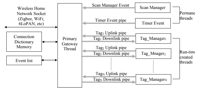
Fig. 1. Software Architecture for Gateway with external network connection socket and connection dictionary memory.
