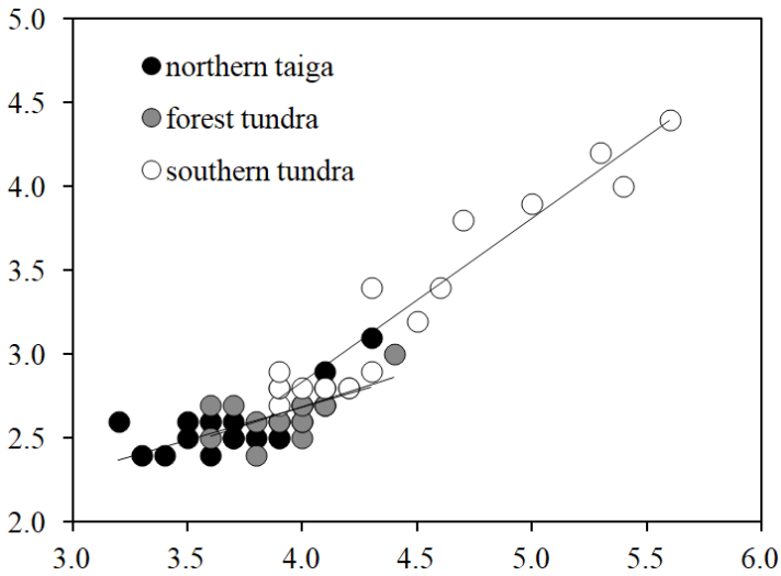
Figure 2. Relationship between \text{pH}_{\text{H}_2\text{O}} values (x-axis) and \text{pH}_{\text{KCl}} (y-axis).
