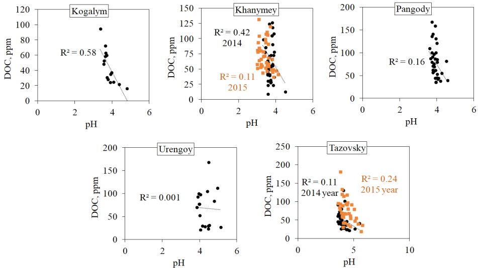
Figure 7. Relationship between DOC content and pH in soil waters of five key sites.
