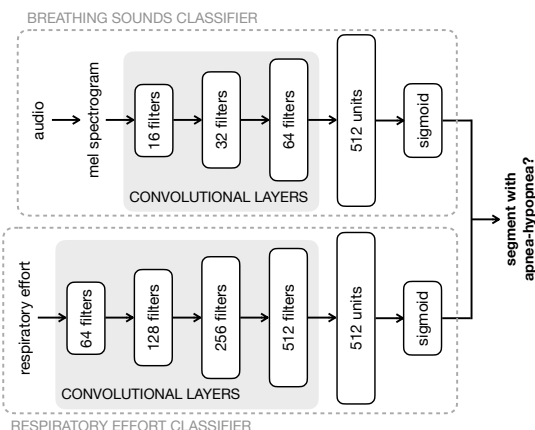
Figure 4: System architecture for late decision fusion
