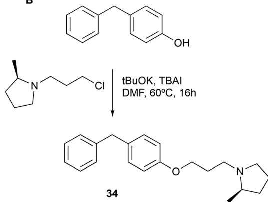
Scheme 3 Synthesis of analogues: (A) 19 and 20 ; (B) 34 .
