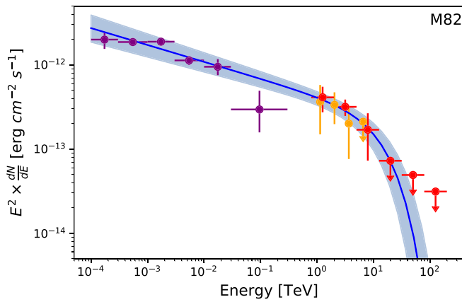
Fig. 25. \gamma -ray spectrum of M82. Data are from Fermi 4FGL-DR2 (purple points, Ballet et al. 2020), from VERITAS (orange points, VERITAS Collaboration et al. 2009), and from ASTRI Mini-Array simulations (100 h, red points). The best fit and its 1\sigma uncertainty are represented by the solid blue line and the shaded region.
