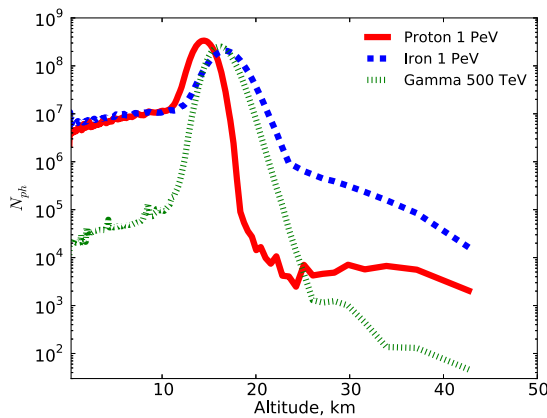
Fig. 39. Simulated longitudinal profile of 1 PeV proton, 1 PeV iron and 500 TeV Gamma-ray at incident angle of 87°. Reproduced from Neronov et al. (2016).
