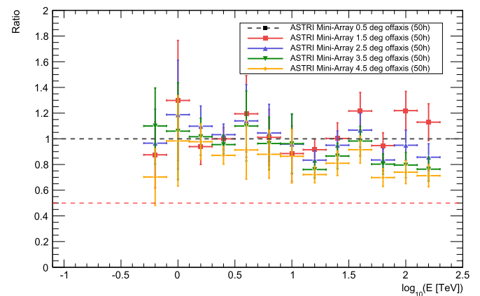
Fig. 6. Top: Off-axis energy resolution of the ASTRI Mini-Array as a function of the energy between 10^{-0.3} \simeq 0.5 TeV and 10^{2.3} \simeq 200 TeV for 5 source off-axis bins between 0^\circ and 5^\circ . Bottom: Energy resolution ratios with respect to the energy resolution achieved in the first considered off-axis bin (from 0^\circ to 1^\circ ). The ratio is calculated so that higher values correspond to better performance. The dashed, thin red line represents a performance drop of a factor 2.
