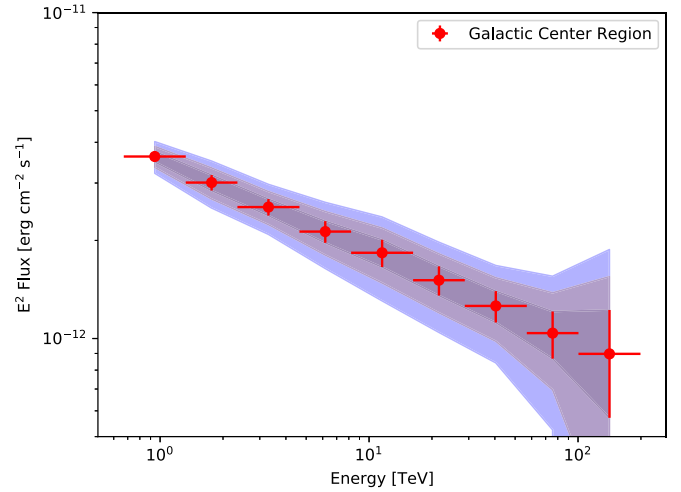
Fig. 46. Simulated spectrum of the Galactic Centre. Red dots show the simulated flux as derived following the procedure described in the text and in Section 5.1.2, Fig. 17. The dashed areas represent the 1\sigma (68%), 2\sigma (95%) and 3\sigma (99.8%) regions of uncertainty.
