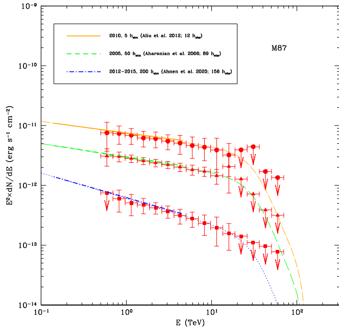
Fig. 28. Same as Fig. 27 for M 87 considering the low (blue lines), high (green lines) and flaring (orange lines) states as reported by MAGIC Collaboration et al. (2020d); Aharonian et al. (2006c); Aliu et al. (2012), and simulating integrations of 5, 50 and 200 h respectively.
