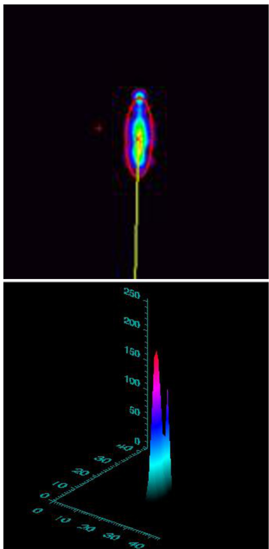
Fig. 37. An event recorded in the ASTRI-Horn camera. As can be seen, both in the 2-D and in the 3-D representations, a single bright pixel is outside the main Cherenkov image.
