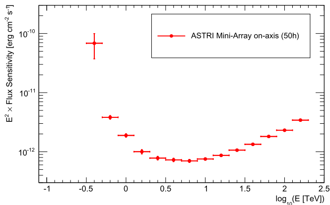
Fig. 4. On-axis differential sensitivity (multiplied by energy squared) of the ASTRI Mini-Array for 50 hours of observations as a function of the energy between \simeq 0.3 TeV and \simeq 200 TeV.
