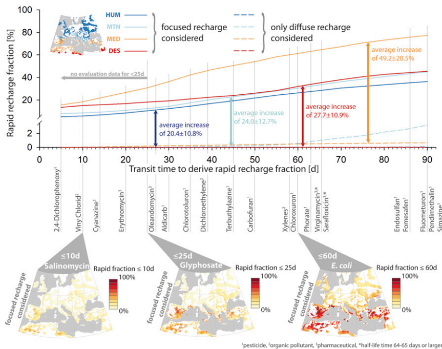
Fig. 3. Rapid recharge fractions of groundwater recharge for transit times of 5 to 90 d for the four simulated regions in relation to 20 example pollutants with varying half-lives ( SI Appendix, Table S4 ), and the spatial distribution of the three example pollutants Salinomycin, glyphosate, and E. coli . Solid lines represent the simulations including focused recharge processes, while dashed lines indicate the rapid recharge fractions that would occur if only diffuse recharge processes were considered. The simulations are most reliable for transit times between the evaluation with glyphosate observations (25 d) and the evaluation with the Young Water Fractions (60 to 90 d). The error of simulated rapid recharge fractions (one SD) due to model parameter uncertainty is 9, 7, 9, and 14% for the HUM, MTN, MED, and DES regions, respectively. The maps show the spatial distribution of rapid recharge fractions corresponding to the half-lives and survival times of Salinomycin, glyphosate, and E. coli when focused recharge is considered.
