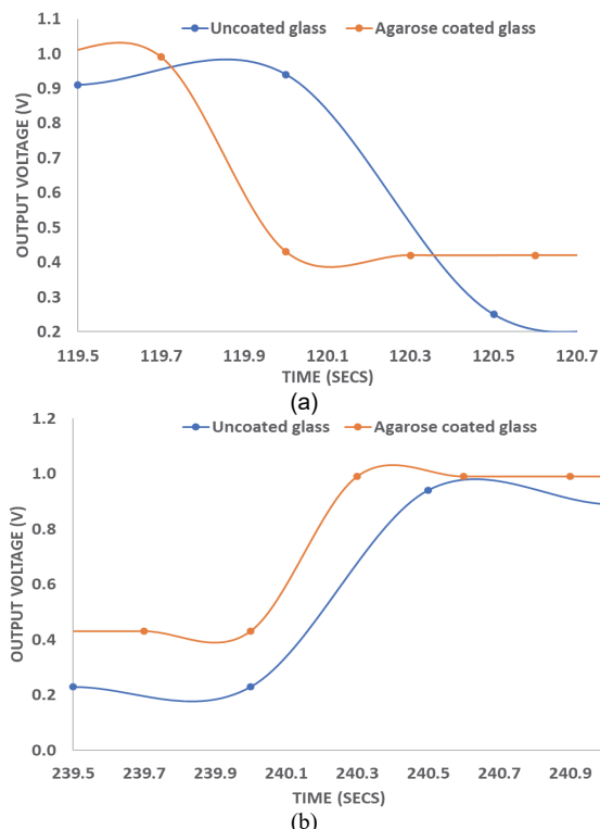
Fig. 7 Time response for both samples; a) Overall, b) Response time and c) Recovery time
