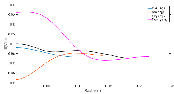
Figure 15. Radial profile of the electric field for a wet poplar sample with a 50% dielectric constant variation between growth rings. Dielectric constant values were used with 0% moisture content according to [27].
