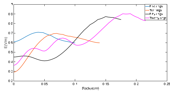
Figure 17. Radial profile of the electric field for a wet poplar sample with a 50% dielectric constant variation between growth rings. Dielectric constant values were used with 28% moisture content according to [27].
