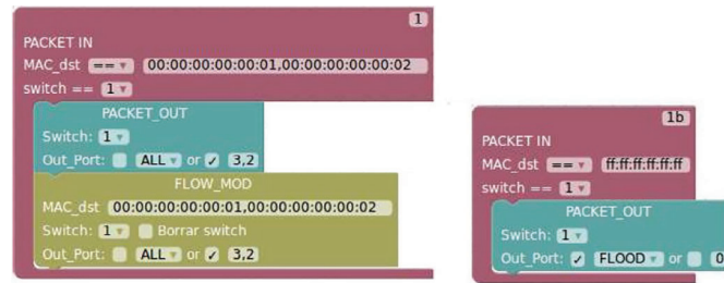
FIGURE 4 Screenshot of ScratchingSDN containing part of the code developed via drag and drop
