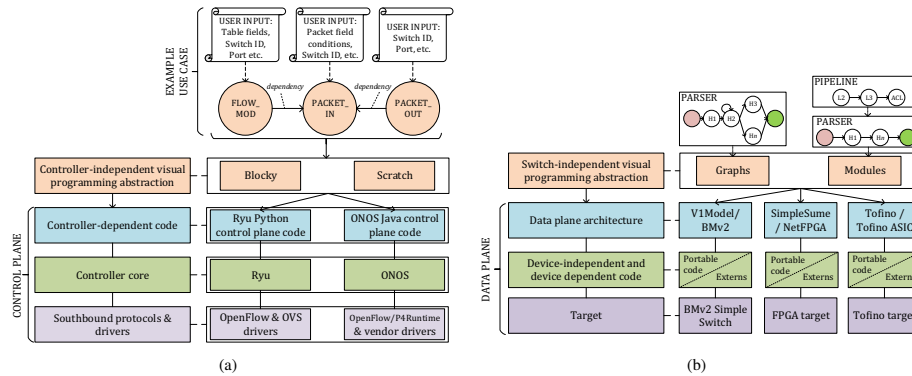
FIGURE 2 Mapping of A, visual abstractions to control plane components, and B, visual abstractions to data plane components
