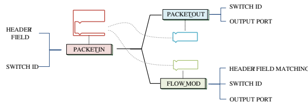
FIGURE 3 Block-based example case. A PACKET_IN handler that outputs PACKET_OUT and FLOW_MOD messages based on user input parameters
