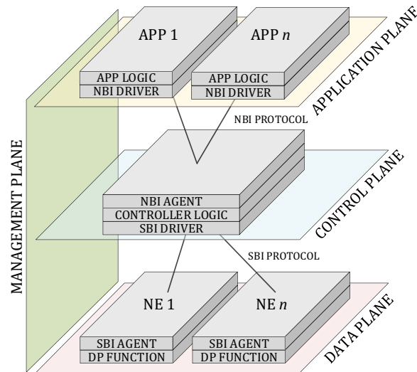
FIGURE 1 A visual representation of the SDN architecture. NE stands for Network Element, APP for Application, NBI for Northbound Interface and SBI for Southbound Interface
