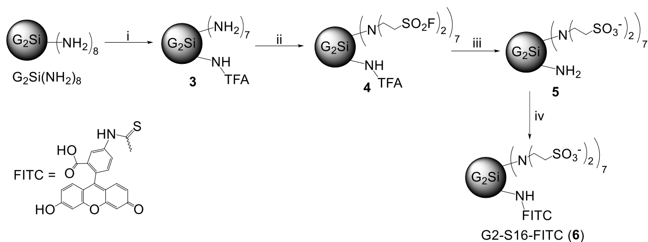
Scheme 2. Synthesis of the anionic sulfonate dendrimer labelled with fluorescein G2-S16-FITC ( 6 ). i) trifluoroacetic anhydride, K 2 CO 3 ; ii) ESF, r. T., 12 h; iii) NaOH, r. T., 4 h; iv) FITC, r. T., 12 h.
