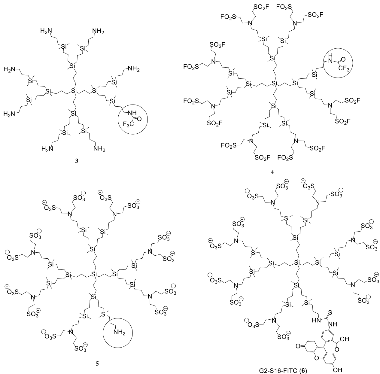
Figure 1. Structure of dendrimers 3-6 . The circle highlights the additional function for labelling of the dendrimer.
