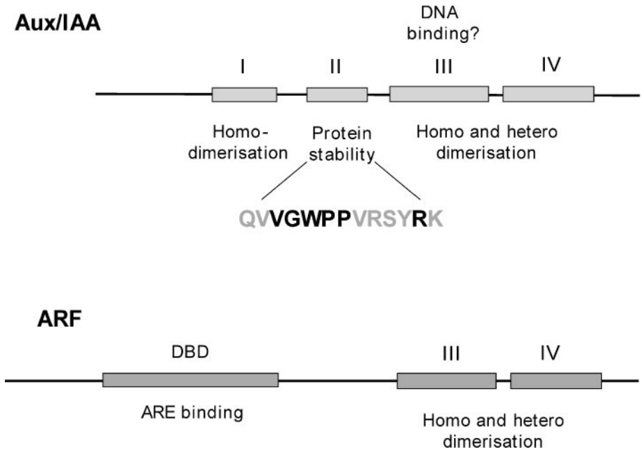
Figure 2 The linear structure of typical family members of the Aux/IAs ( top ) and auxin response factors (ARFs) ( bottom ). The proteins share homology at their carboxyl termini in two domains (III and IV), which mediate homo- and heterodimerization. At the amino terminus, Aux/IAA proteins have two domains, one of which (II) is necessary and sufficient to mediate auxin-regulated destabilization of the protein. The consensus sequence of this domain is shown, with the invariant amino acids in black. ARFs have an amino-terminal DNA binding domain that binds to the auxin response elements (AREs) of auxin-regulated genes.
