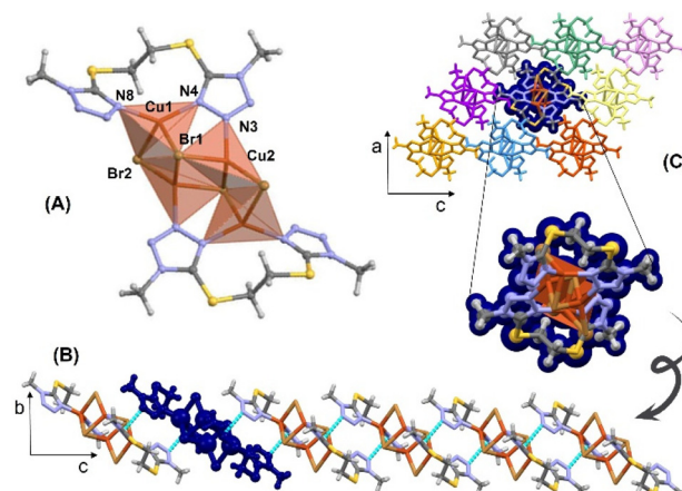
Fig. 4 The molecular structure of 3 (A) showing in detail the C–H \cdots N interactions in the bc plane (B) and the final arrangement in the ac plane (C).
