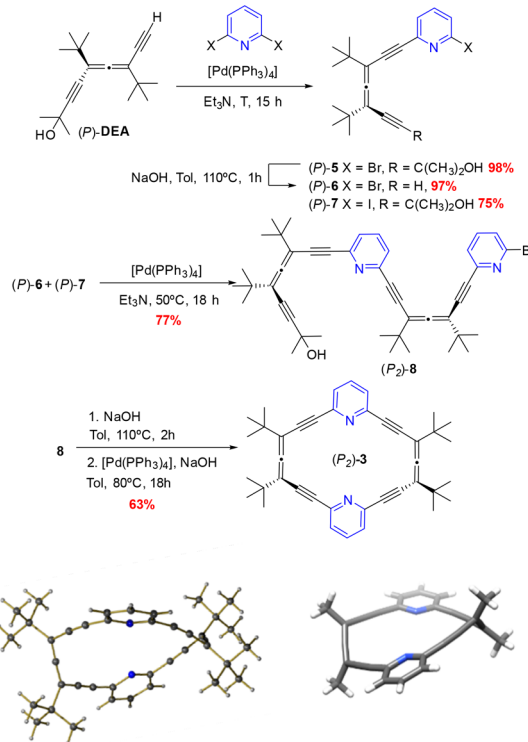
Scheme 1 Synthetic sequence followed to obtain macrocycle 3 . Bottom: Crystal structure resolved by X-ray diffraction ( (P_2) - 3 ) and conformation obtained by DFT computations (CAM-B3LYP/6-31g+(d,p)).
