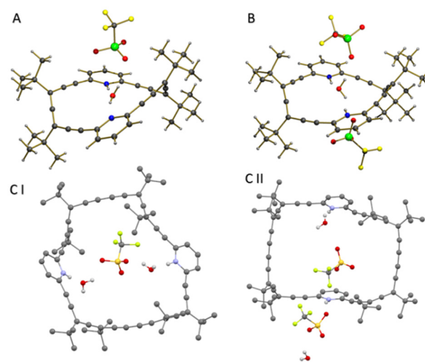
Fig. 3 (A) Crystal structure of 3\cdot\text{H}_2\text{O}\cdot\text{OTf} . (B) Crystal structure of 3\cdot(\text{H}_2\text{O}\cdot\text{OTf})_2 . (C) Crystal structure of 4\cdot(\text{H}_2\text{O}\cdot\text{OTf})_2 : asymmetric units I and II. Hydrogens were omitted for clarity.
