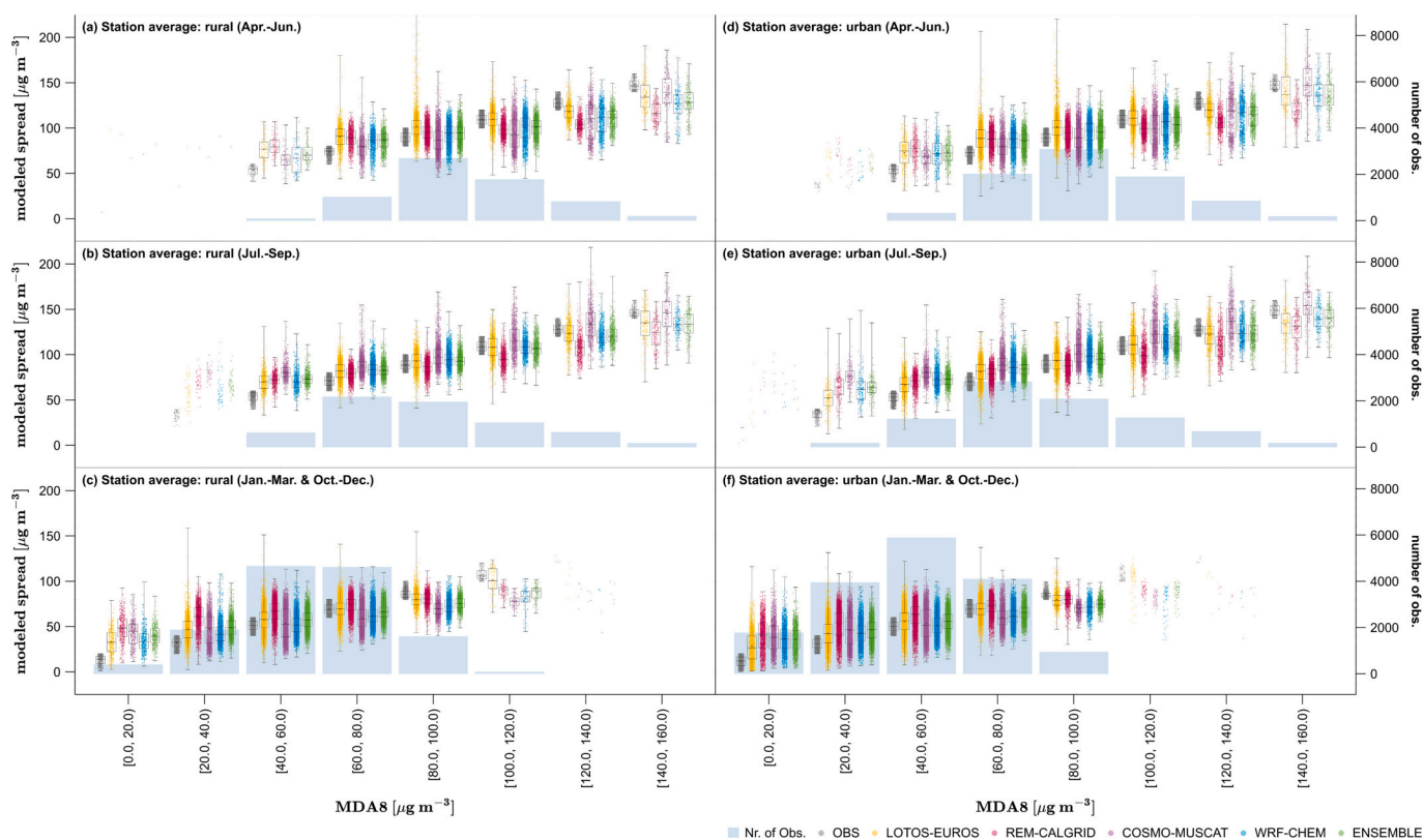
Fig. 4. Modeled ozone concentration (MDA8 \text{O}_3 ) in relation to the measured ozone levels for LOTOS-EUROS (yellow), REM-CALGRID (magenta), COSMO-MUSCAT (purple), WRF-Chem (blue) and the ensemble (green). Observations are shown in grey. Plotted values are binned by the measured background concentration levels of all available monitoring sites in Germany. Each single dot represents one observation (one day of the MDA8 \text{O}_3 in the corresponding bin from one station). The box plot shows the mean, median, 25 th and 75 th percentile as well as the min and max values. Different station classes are separated out for rural (a–c) and urban (d–f) areas. The periods of April–June and July–September are shown in the subplots (a,d) and (b,e) as well as the winter months January–March and October–December in subplots (c,f).
