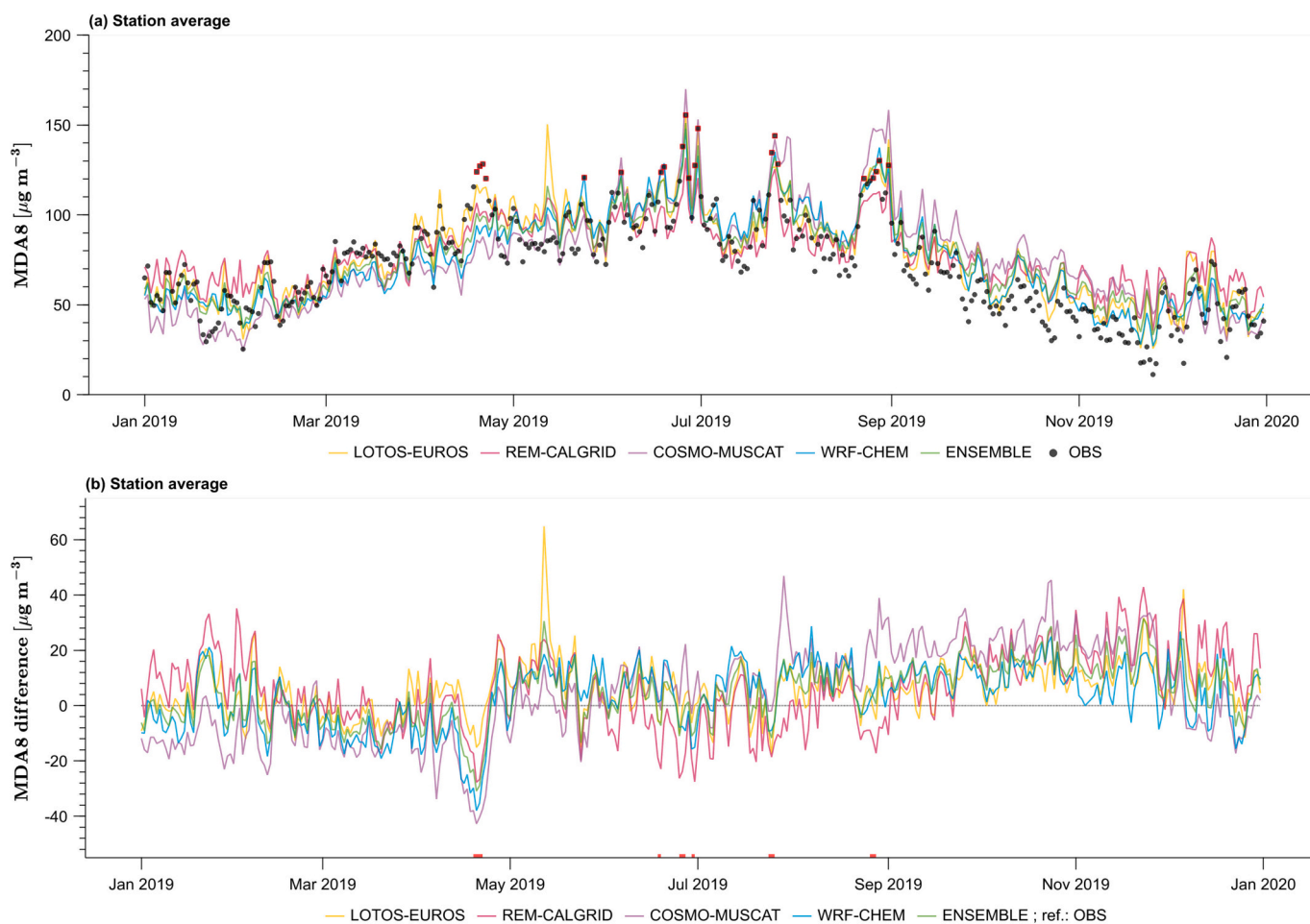
Fig. 3. Time series (a) of the MDA8 \text{O}_3 for LOTOS-EUROS (yellow), REM-CALGRID (magenta), COSMO-MUSCAT (purple), WRF-Chem (blue) and the ensemble mean (green). Plotted values reflect the average background concentration of all available monitoring sites in Germany. Measured concentrations are indicated with black circles. The difference for each model and the ensemble mean to the measured concentration is shown in subplot (b). Exceedances above the MDA8 \text{O}_3 target value of 120 \mu\text{g m}^{-3} are indicated with red dots.
