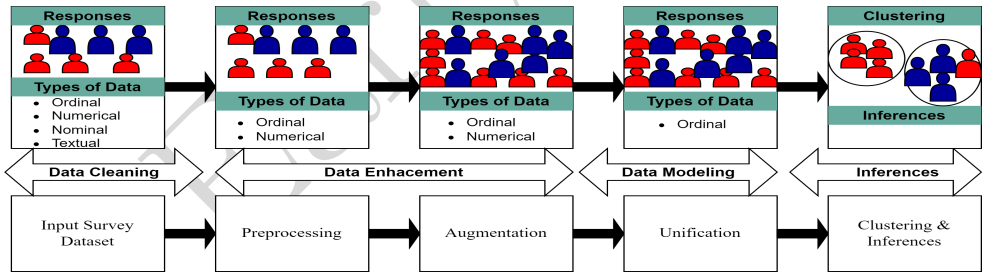
Figure 2. Workflow of the Proposed Methodology.
