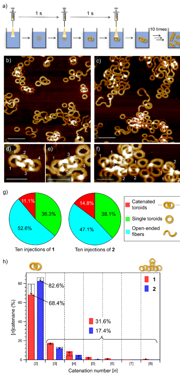
Fig. 4 (a) Depiction of the portion-wise solvent-mixing protocol. (b and c) AFM images of supramolecular polymers obtained by injecting a 100 \mu\text{L} chloroform solution ( c = 1.0 \times 10^{-3} M) of 1 (b) or 2 (c) into 900 \mu\text{L} of MCH in ten portions (one injection per second). Scale bars, 100 nm. Catenated toroids are shown in red dotted circles. (d–f) AFM images of the nano-[4]catenane of 1 (d and e) and nano-[2]catenane of 2 (f). Scale bars, 50 nm. (g) Pie charts showing the yields of catenanes (red), single toroids (green), and open-ended fibers (light blue) in MCH from a portion-wise solvent-mixing experiment. The numbers of sampled toroids are 1478 and 1419 for 1 and 2 , respectively. (h) Bar charts showing the percentages of oligomeric nano-[ n ]catenanes ( n = 2 –8) of 1 (red) and 2 (blue) obtained by portion-wise injections. Overlapped black dotted bars indicate the percentages of nano-[ n ]catenane obtained by single-injection shown in Fig. 1g.
