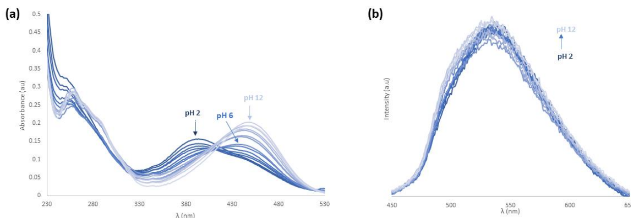
Fig. 9: (a) Representative UV-Vis pH titration of L2 with additions of \text{NaOH}_{(\text{aq})} at 0.1 pH unit intervals and an initial \text{CH}_3\text{COOH}_{(\text{aq})} acid spike. (b) Representative fluorescence pH titration ( \lambda_{\text{ex}} = 400\text{nm} ) with additions of \text{NaOH}_{(\text{aq})} and an initial \text{CH}_3\text{COOH}_{(\text{aq})} acid spike in \text{H}_2\text{O} medium.
