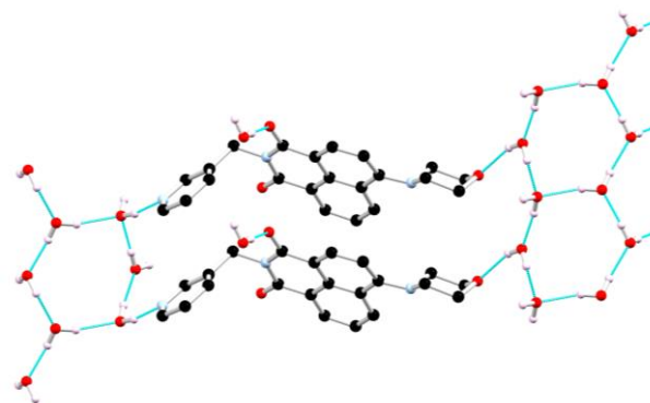
Fig. 2: Extended structure of L1 featuring hydrogen bonding and \pi - \pi stacking interactions between adjacent ligand moieties. Hydrogen atoms not involved in hydrogen bonding are omitted for clarity.
