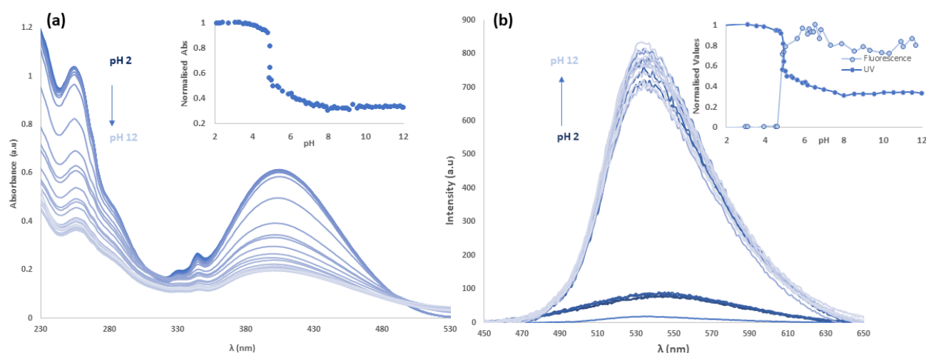
Fig. 8: (a) UV-Vis pH titration of L1 with \text{NaOH}_{(\text{aq})} at 0.1 pH unit intervals and an initial \text{HCl}_{(\text{aq})} acid spike in 100 mM \text{NaCl}_{(\text{aq})} medium. (insert) Normalised absorbance ( \lambda_{\text{max}} = 400\text{ nm} ) of the titration. (b) Fluorescence pH titration of L1 with \text{NaOH}_{(\text{aq})} at 0.1 pH unit intervals and an initial \text{HCl}_{(\text{aq})} acid spike in 100 mM \text{NaCl}_{(\text{aq})} medium. (Insert) Normalised absorbance ( \lambda_{\text{max}} = 400\text{ nm} ) and fluorescence of the titration ( \lambda_{\text{ex}} = 400\text{ nm} , \lambda_{\text{max}} = 550\text{ nm} ).
