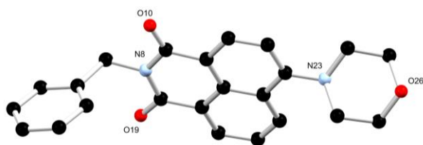
Fig. 5: Structure of L2 with heteroatom labelling scheme. All hydrogen atoms are omitted for clarity.
