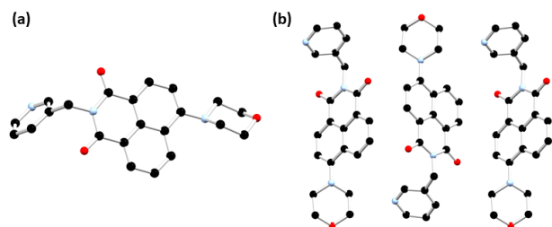
Fig. 3: (a) Structure of L1-gel from dissolution of the gel sample. Hydrogen atoms are omitted for clarity. (b) Extended structure of L1 featuring offset head-to-tail \pi\cdots\pi stacking interactions between adjacent naphthalimide rings. Hydrogen atoms are omitted for clarity.
