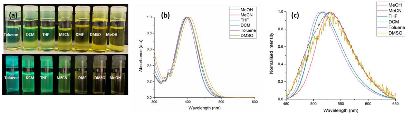
Fig. 7: (a) Corresponding photograph taken in room light and under UV light, (b) UV absorption spectra of L1 in solvents of varying polarity (c) Normalised fluorescence spectra of L1 in solvents of varying polarity.
