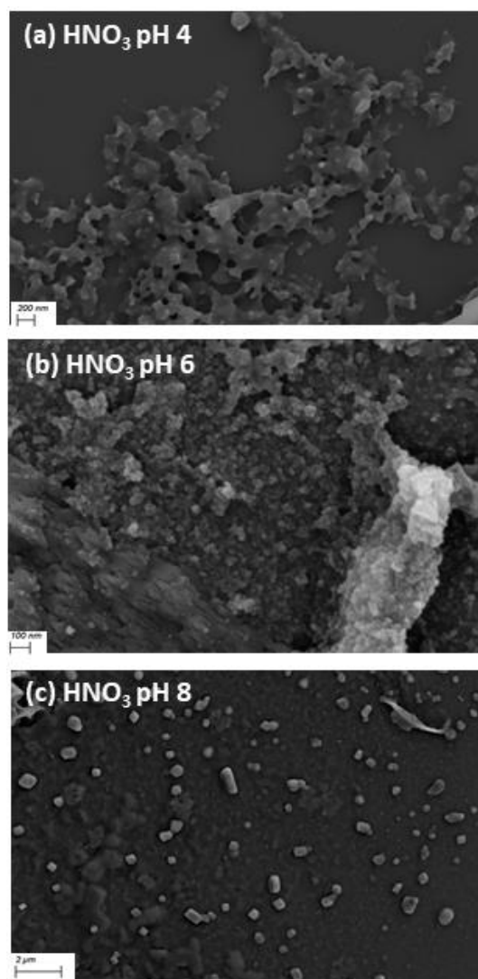
Fig. 10: (a) SEM image of L2 sample spiked with \text{HNO}_3 at pH4 showing a branching morphology of aggregates, (b) SEM image of L2 sample spiked with \text{HNO}_3 at pH6 showing a higher density of aggregates (c) SEM image of L2 sample spiked with \text{HNO}_3 at pH8 showing micrometer aggregates.
