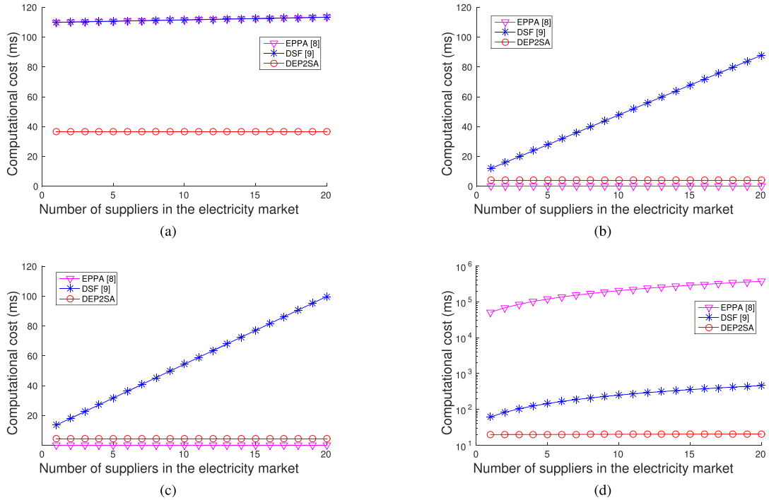
FIGURE 10. Computational cost comparison at a BG, NG, WG and DCC. (a) At each BG. (b) At each NG. (c) At each WG. (d) At the DCC.
