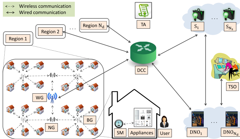
FIGURE 2. A multi-recipient system model (architecture) used in the design of DEP2SA.
