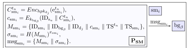
FIGURE 4. SM report generation: the P_{SM} processing step.
