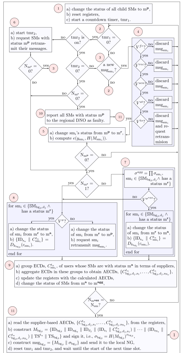
FIGURE 5. A flowchart of the operations at a BG: the P_{BG} processing step.
