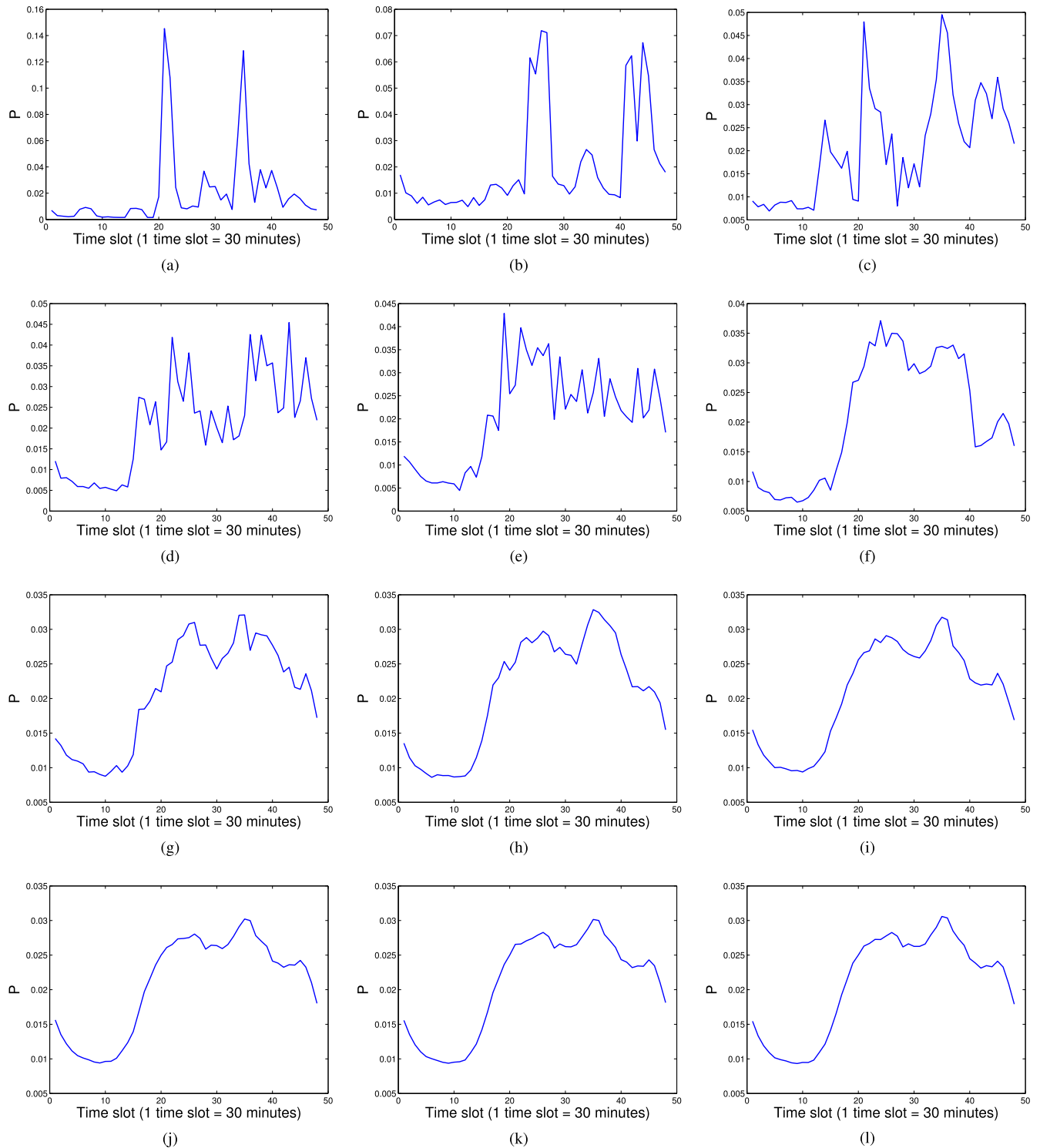
FIGURE 8. The ACD distributions of subsets with an increasing number of users from a dataset, i.e., P_{\Sigma(\mathbb{E}_1^{t_n})} (8a), ..., P_{\Sigma(\mathbb{E}_{5000}^{t_n})} (8k), and the ACD distribution of all the users in the dataset, i.e., P_{\Sigma(\mathbb{E}_{6287}^{t_n})} (8l), over a 24-hour period. (a) N_{sm} = 1 , K = 1.08 \times 10^{-1} . (b) N_{sm} = 2 , K = 5.97 \times 10^{-2} . (c) N_{sm} = 5 , K = 2.17 \times 10^{-2} . (d) N_{sm} = 10 , K = 1.59 \times 10^{-2} . (e) N_{sm} = 20 , K = 7.92 \times 10^{-3} . (f) N_{sm} = 50 , K = 5.61 \times 10^{-3} . (g) N_{sm} = 100 , K = 7.82 \times 10^{-4} . (h) N_{sm} = 300 , K = 7.30 \times 10^{-4} . (i) N_{sm} = 1000 , K = 1.66 \times 10^{-4} . (j) N_{sm} = 3000 , K = 1.83 \times 10^{-5} . (k) N_{sm} = 5000 , K = 8.85 \times 10^{-6} . (l) N_{sm} = 6287 , K = 0 .
