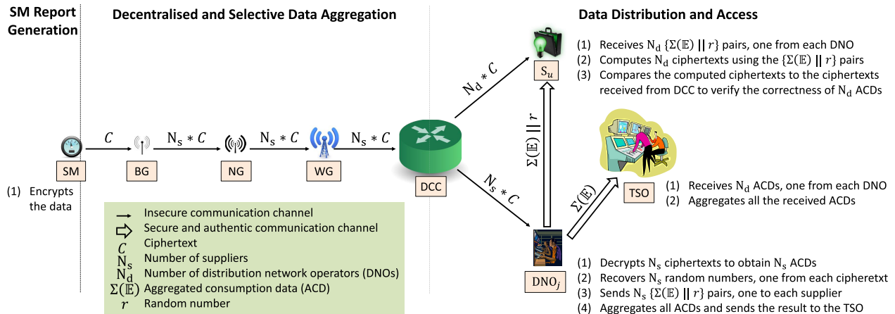
FIGURE 3. An overview of DEP2SA.
