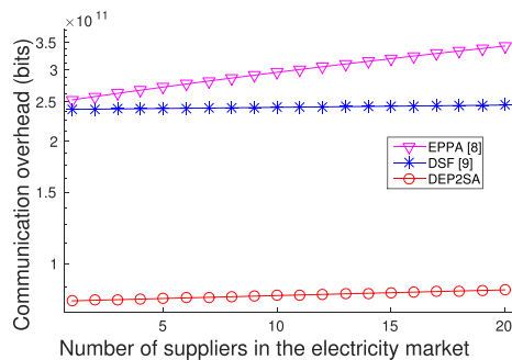
FIGURE 12. Communication overhead comparison at the SMS-to-DCC part.
