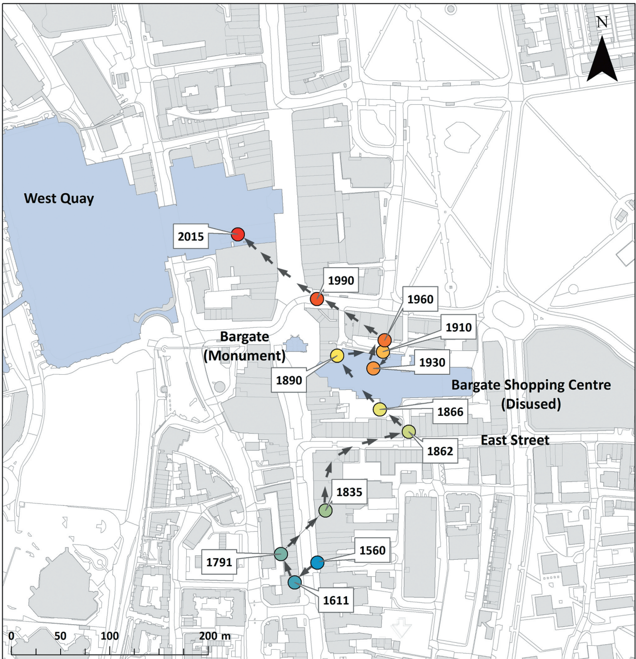
Figure 4. Position of the city center centroids through time overlaid on a current map. Main background features are highlighted in light blue and other buildings are shown in light gray.
