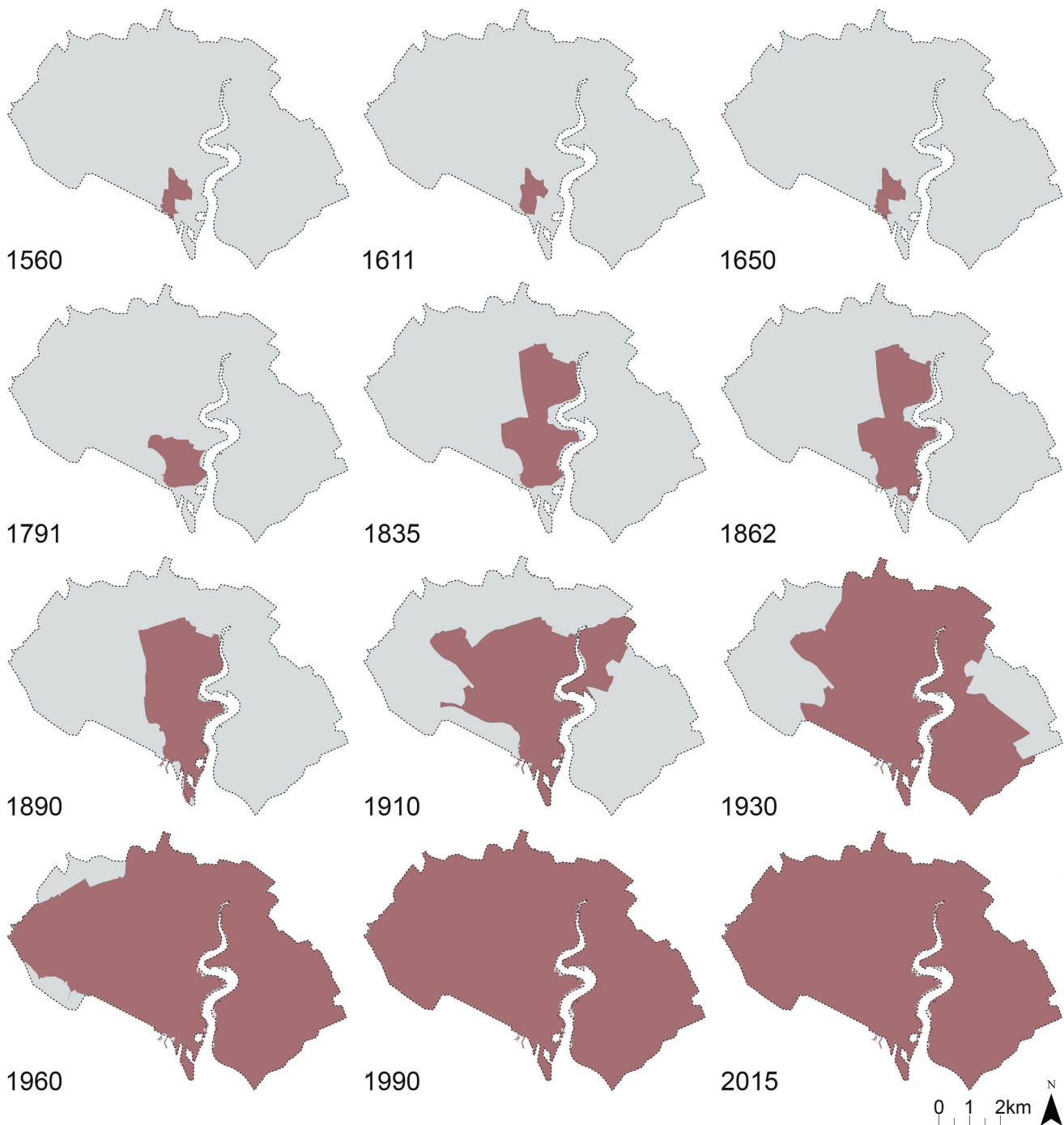
Figure 3. Evolution of Southampton's urban boundary (1560–2015). The brown shaded area shows the boundary at the time superimposed on the extent of modern-day Southampton city. Scale bar and north arrow in all years as for 2015. For detailed maps, see Appendix A in Supplementary Materials.
