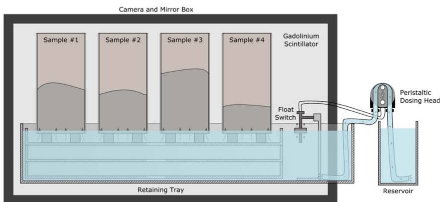
Fig. 3 Illustration of the configuration of the experiment in the NEUTRA instrument. The water level was maintained by the peristaltic dosing head activated by the float switch when the water level dropped.
