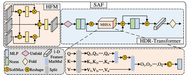
Figure 3: The architecture of the proposed module Self-Attention Fusion (SAF) in PFM, which is composed of the HDR Fusion Module and HDR Transformer, respectively. The bottom in the figure is Multi-Head Self Attention.
