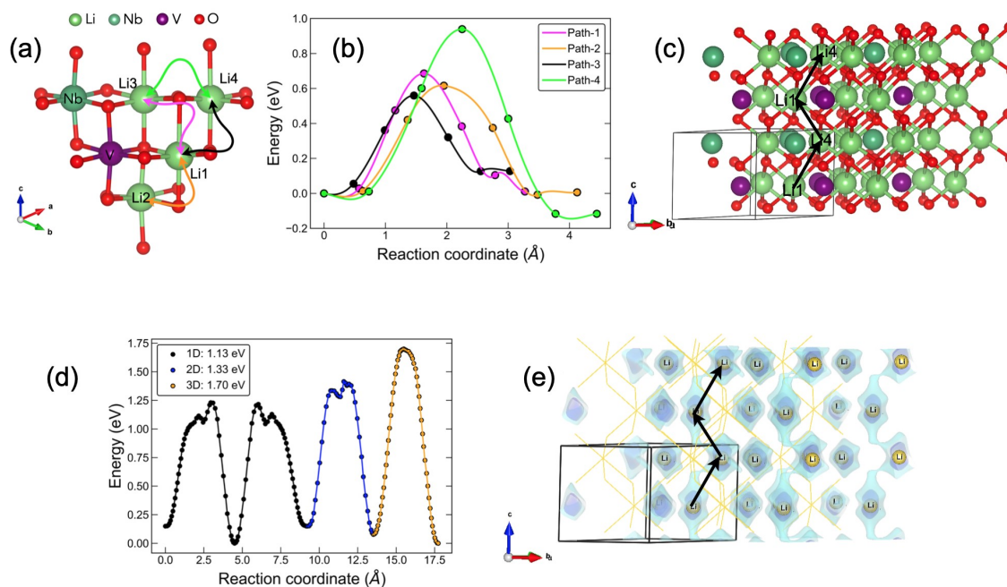
Fig. 8 Schematic overview of the \text{Li}^+ diffusion in \text{Li}_4\text{NbVO}_6 . (a) Unit cell of \text{Li}_4\text{NbVO}_6 showing all possible elementary \text{Li}^+ hops colored according to their diffusion barriers. (b) DFT-CI-NEB computed energy barriers where the different colors correspond to the elementary jumps shown in (a). (c) The long-range minimum energy pathway for \text{Li}^+ ( \text{Li1} \leftrightarrow \text{Li4} ) is shown in a 2 \times 2 \times 2 supercell identified to be along the (001) direction marked by black arrows. (d) BVSE computed \text{Li}^+ migration pathway for 1D, 2D, and 3D percolation network with corresponding activation barriers. (e) 3D network of \text{Li}^+ pathways (blue isosurface) calculated by BVSE. The minimum energy pathway for \text{Li}^+ migration is identified to be along the (001) direction (marked by black arrows) and matches exactly with the CI-NEB results shown in (c).
