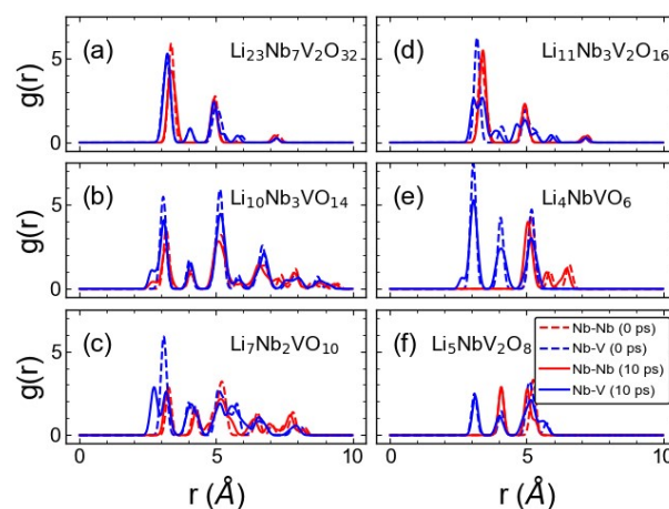
Fig. 9 Radial distribution function plots. Radial distribution function between Nb-Nb (red) and Nb-V (blue) of (a) \text{Li}_{23}\text{Nb}_7\text{V}_2\text{O}_{32} (b) \text{Li}_{10}\text{Nb}_3\text{VO}_{14} (c) \text{Li}_7\text{Nb}_2\text{VO}_{10} (d) \text{Li}_{11}\text{Nb}_3\text{V}_2\text{O}_{16} (e) \text{Li}_4\text{NbVO}_6 and (f) \text{Li}_5\text{NbV}_2\text{O}_8 structures at 0 ps (dashed line) and 10 ps (solid line) obtained from AIMD simulations at 600 K.
