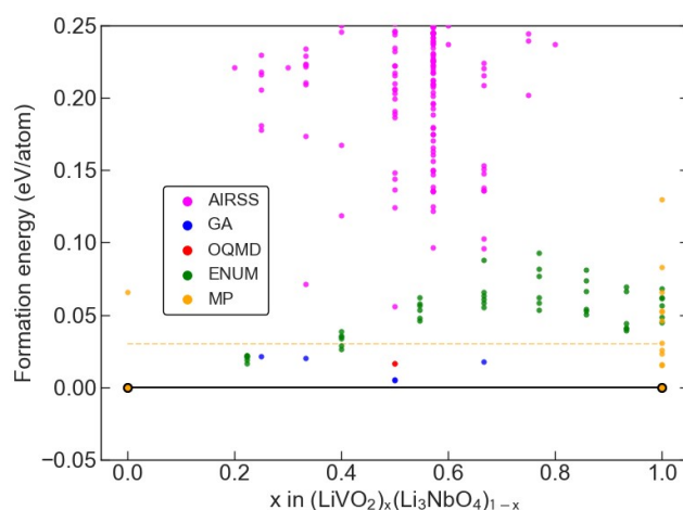
Fig. 2 Convex hull diagram. Convex hull plot along the pseudobinary tieline of \text{LiVO}_2 and \text{Li}_3\text{NbO}_4 showing the formation energy (eV/atom) versus composition along the tieline. The different colors represent the different data sources. The dashed horizontal line is the 30 meV/atom limit on the formation energy, which we take as the 0K thermodynamic limit.
