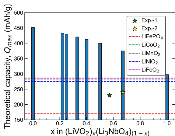
Fig. 4 Theoretical capacity as a function of composition. Theoretical capacity as a function of composition along the \text{LiVO}_2 - \text{Li}_3\text{NbO}_4 tieline. Exp.-1 and Exp.-2 values are taken from Ref. 21 and Ref. 23 , respectively.
