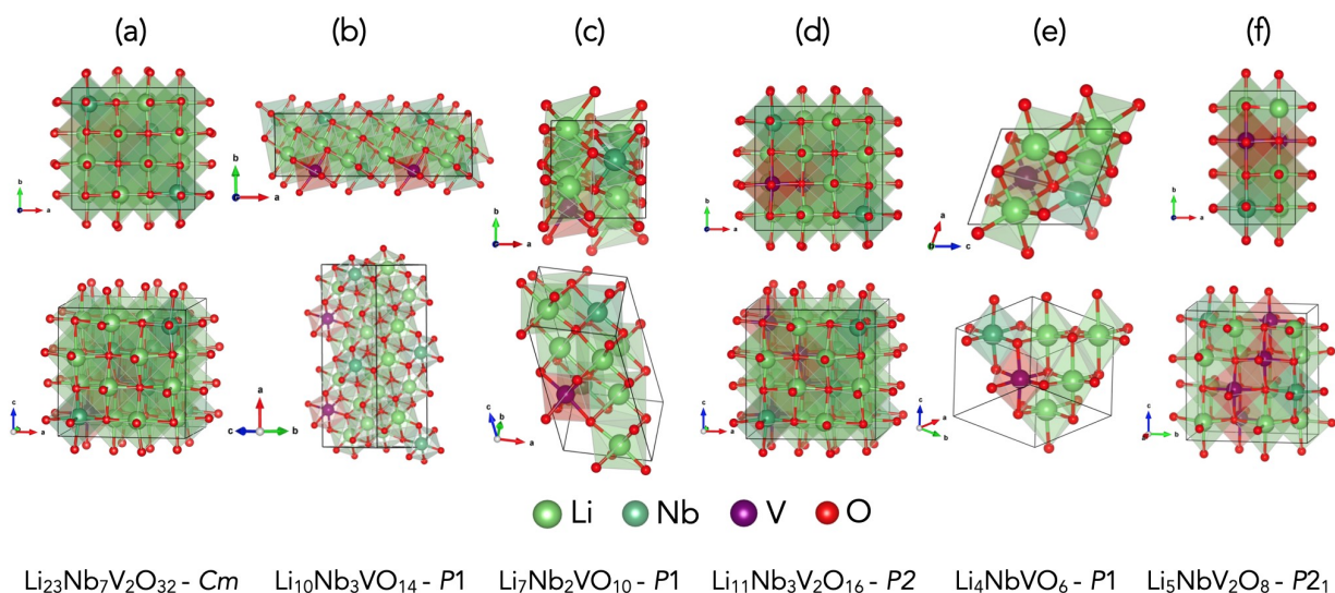
Fig. 3 Predicted ground state crystal structures. Ground state crystal structures found by different crystal structure prediction algorithms whose formation energy value lies within 30 meV/atom from the convex hull of \text{LiVO}_2 - \text{Li}_3\text{NbO}_4 pseudobinary tieline.
