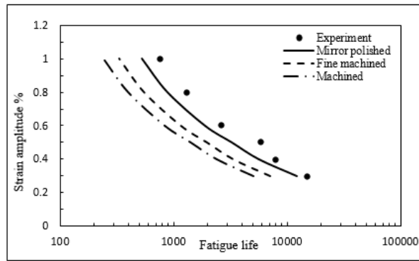
Fig.6. Obtained fatigue life by Fe-Safe employing Brown-Miller and Roy et al. [48] experiment.
