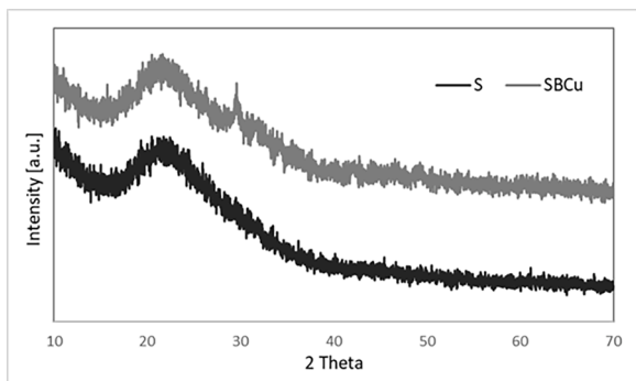
Fig. 5. XRD patterns of S and SBCu glasses.
