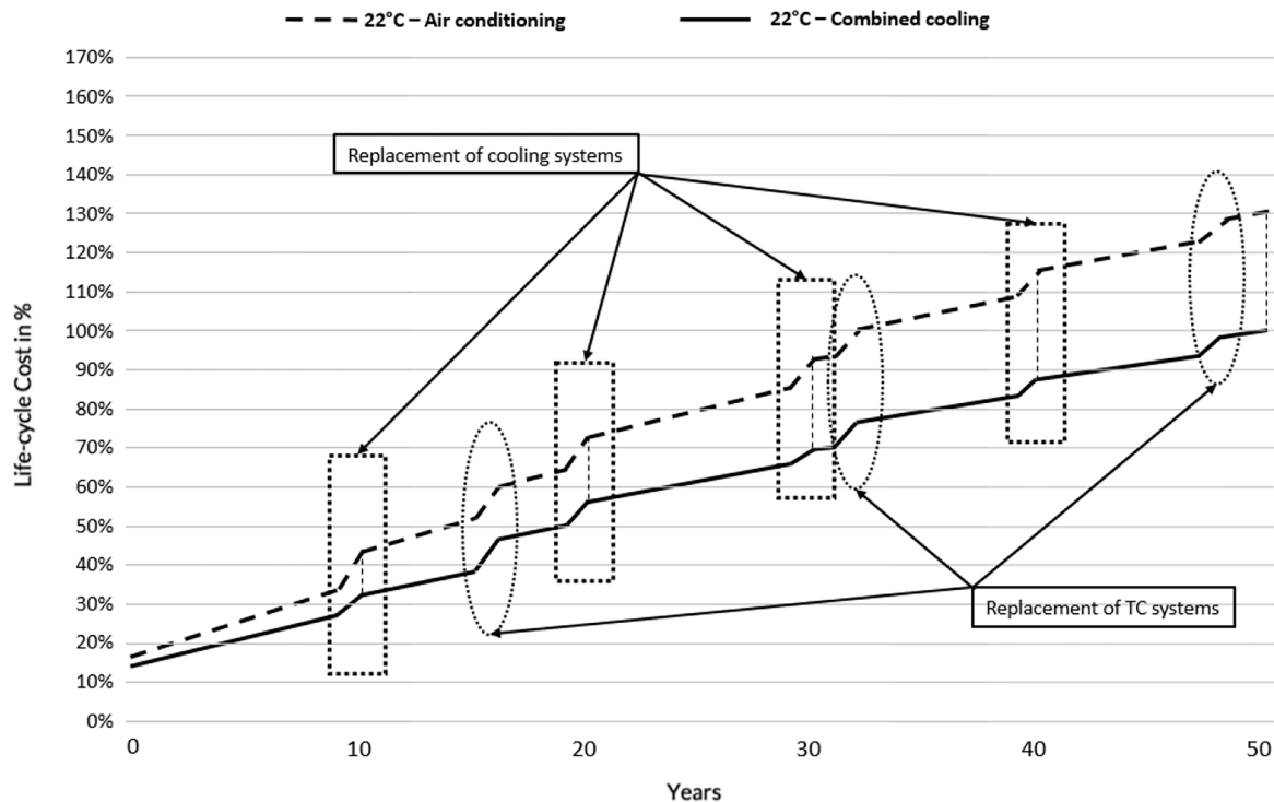
Fig. 14. Comparison of life cycle cost for a combination of ventilation and air conditioning and for full equipment with air conditioning (active cooling) units ((Fruhwirt, 2021), data originally published in (Scherz et al., 2019)).
