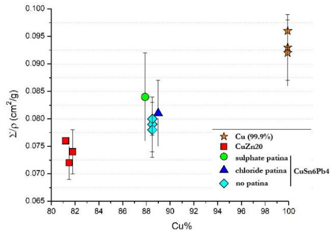
Figure 7. Evaluation of attenuation mass coefficient according to different composition (pure Cu and CuZn alloy with Zn 20 wt%); some preliminary results obtained on coated samples (CuSn6Pb4) are also represented in function of the attenuation mass coefficient.
