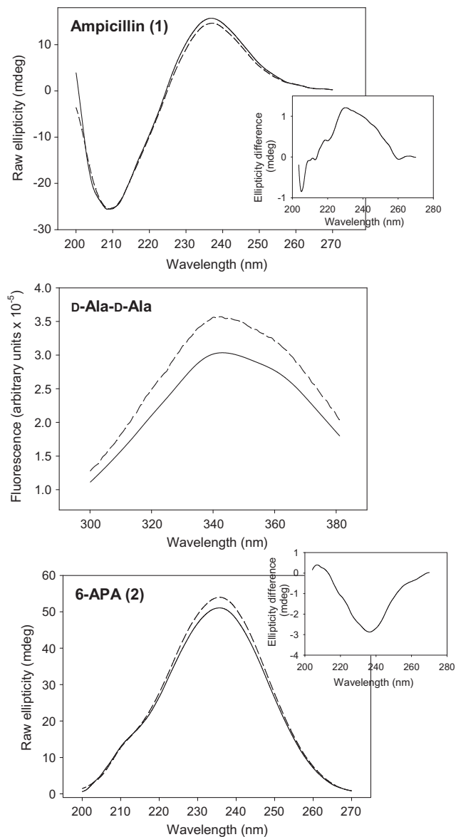
Fig. 5. Upper panel: Interaction of 5.6 \mu M C-StkP with 1 mM ampicillin ( 1 ) monitored by CD at 25 ^{\circ} C in 20 mM sodium phosphate, 50 mM NaCl, pH 7.0; the solid line is the experimental spectrum of the complex, and the dashed line is the theoretical spectrum obtained by the sum of the spectra of protein and ligand recorded separately. The inset shows the difference in ellipticity between experimental and theoretical spectra. Experiments were repeated four independent times and a typical result is shown in the figure. Middle panel: Intrinsic fluorescence spectrum of 5.6 \mu M C-StkP (solid line) and 5.6 \mu M C-StkP plus 1 mM D-Ala-D-Ala (dashed line). Lower panel: Interaction of 5.6 \mu M C-StkP with 1 mM 6-APA ( 2 ) monitored by CD. Conditions and line patterns as in the upper panel.
