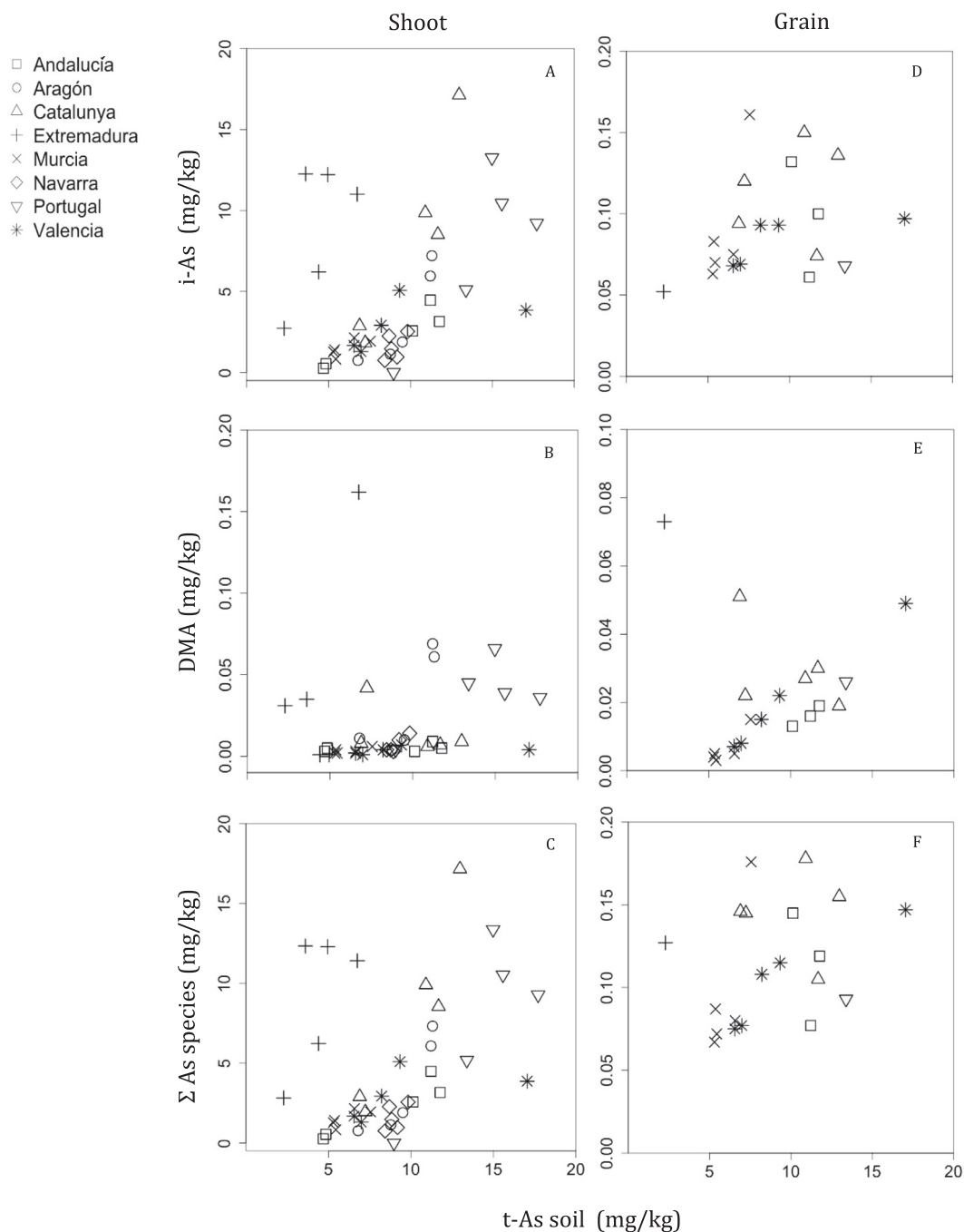
Fig. 2. Relationship between t-As concentration (mg/kg dry weight) in soil and i-As, DMA and \Sigma As concentration (mg/kg dry weight) in rice tissues (shoots and field-collected rice grains) according to paddy field region.
