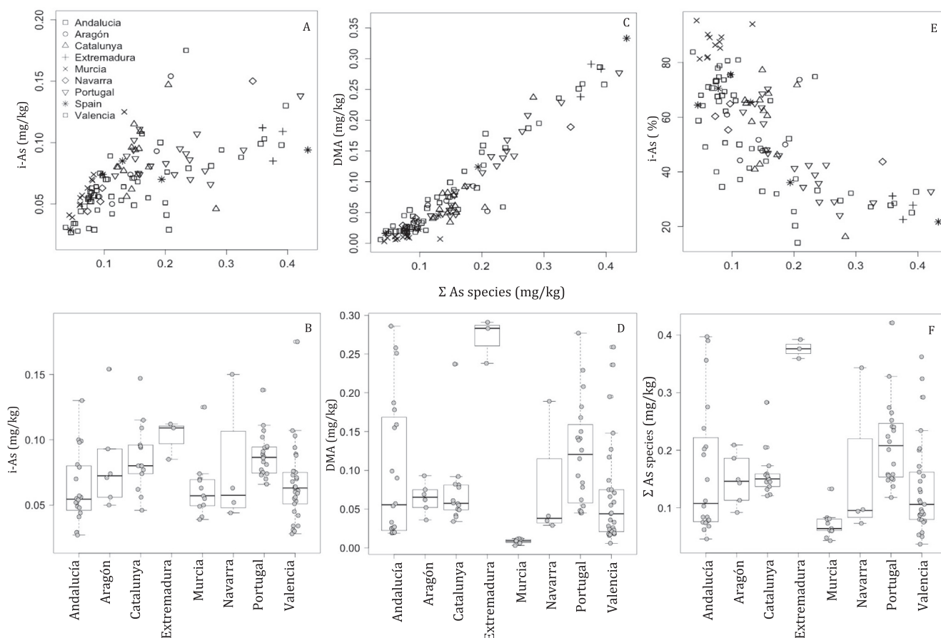
Fig. 4. Relationship between \Sigma As and i-As, DMA concentration (mg/kg dry weight) and i-As (%), and i-As, DMA and \Sigma As concentration (mg/kg dry weight) in commercial polished rice according to paddy field region.
