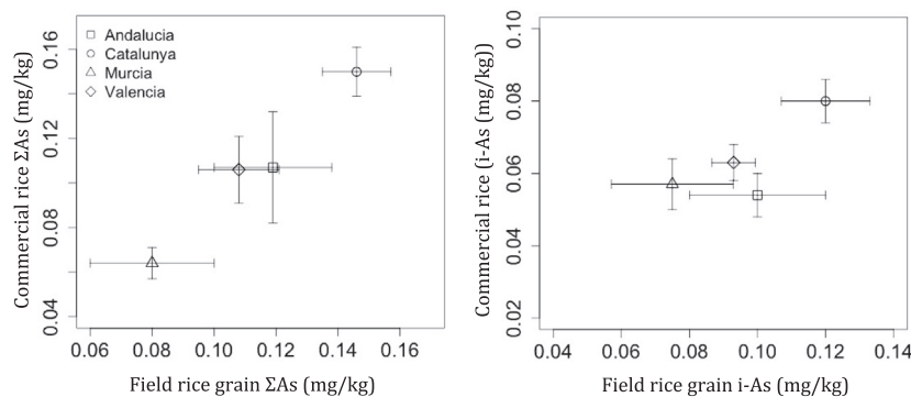
Fig. 3. Relationship between polished commercial rice and field-collected rice grain i-As and \Sigma As concentration (mg/kg dry weight). Each value shows the median and standard error according to paddy field region.
