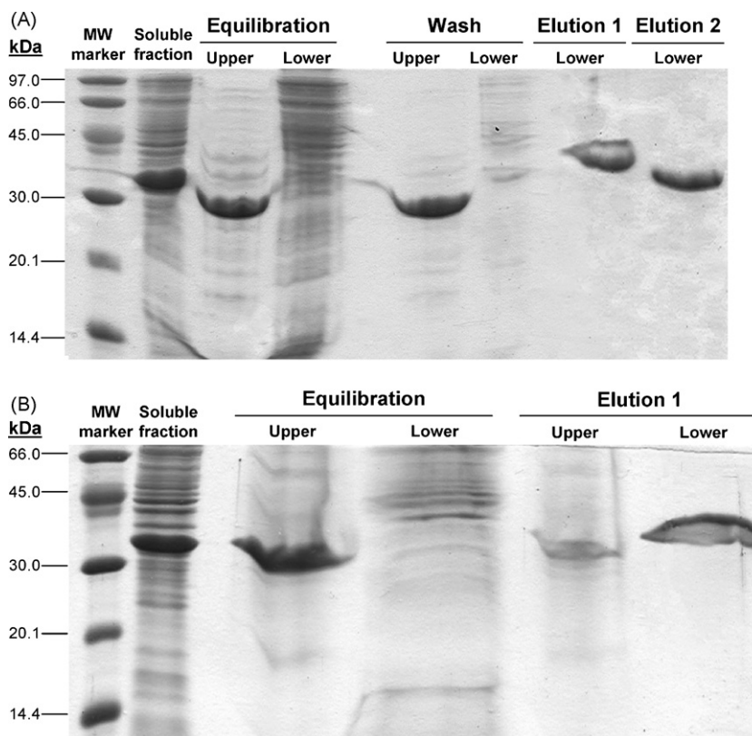
Fig. 8. (A) Purification of C-LytA-ProtA in PEG/phosphate. (B) Purification of C-LytA-ProtA in PEG/dextran.
