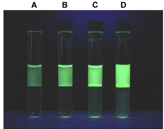
Fig. 4. Effect of extract concentration on the partition properties of GFP-C-LytA in PEG/phosphate. (A) 0.45 mg/ml; (B) 0.9 mg/ml; (C) 1.9 mg/ml; (D) 4.0 mg/ml. Samples were illuminated with UV light in order to induce GFP fluorescence.
