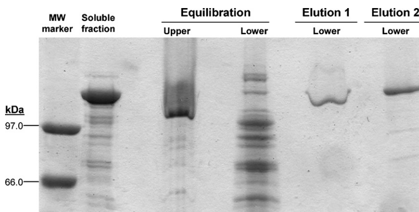
Fig. 7. Purification of LYTAG-β-galactosidase in PEG/dextran from E. coli REG-1 [pALEX2c-LacZ]. SDS-PAGE was Coomassie stained.
