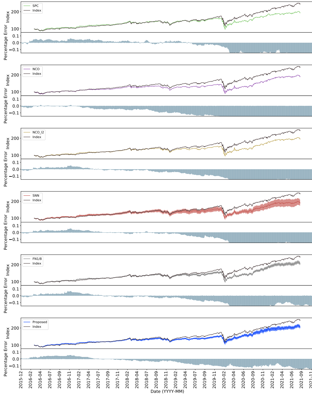
Figure 10: Index tracking performance for different methods based on S&P 500 index. From up to the bottom are SPC, NCO, NCO_{\ell_2} , SNN, FN1/8, and our proposed methods, respectively. For every single plot, the top plots are the index and the trackers, and the bottom is the percentage tracking error \frac{\hat{y} - y}{y} . Shadow area covers one standard deviation for SNN, FN1/8, and our proposed method.
