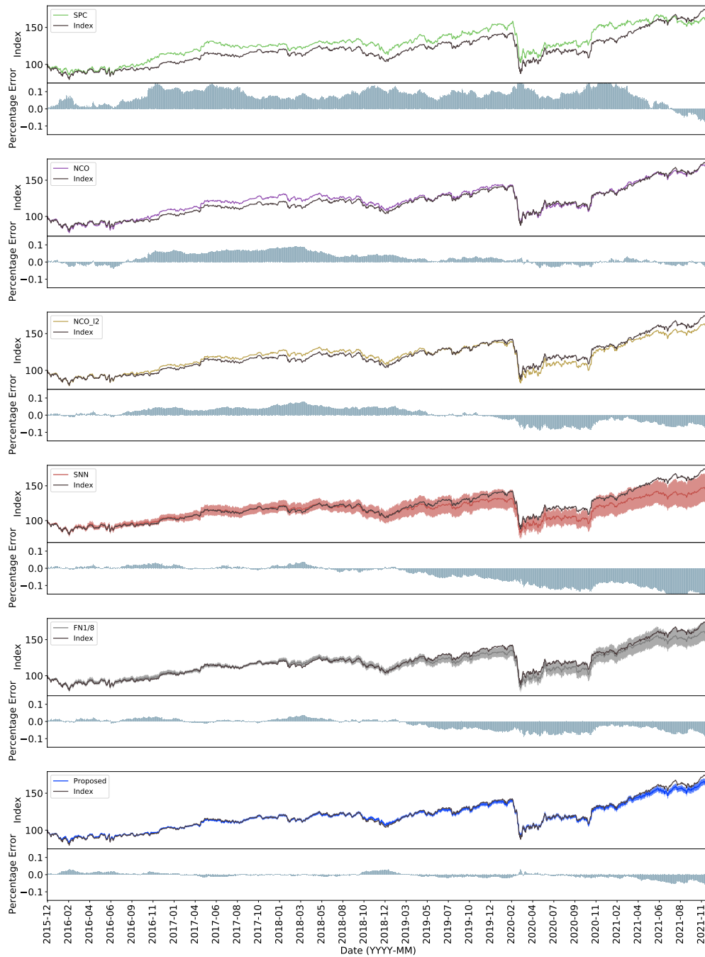
Figure 8: Index tracking performance for different methods based on CAC 40 index. From up to the bottom are SPC, NCO, NCO l2 , SNN, FN1/8, and our proposed methods, respectively. For every single plot, the top plots are the index and the trackers, and the bottom is the percentage tracking error \frac{\hat{y}-y}{y} . Shadow area covers one standard deviation for SNN, FN1/8, and our proposed method.
