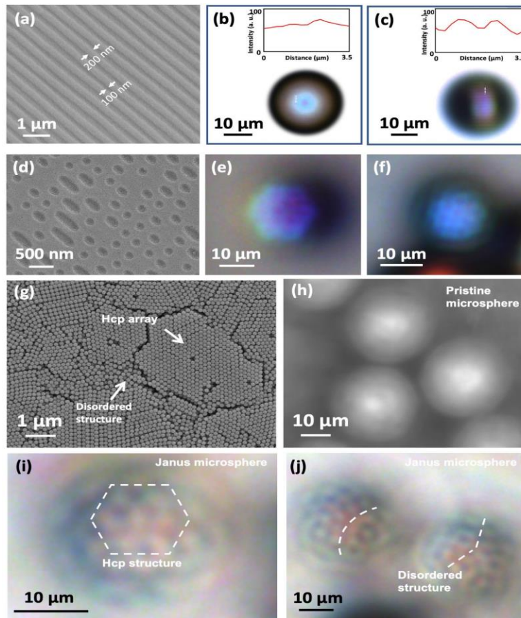
Fig. 2. (a) Scanning electron microscopic (SEM) image of a BD; (b), (c) OM pictures of the BD observed through (b) a pristine microsphere and (c) a Janus microsphere; (d) SEM image of a BD with data pits; (e), (f) OM pictures of the BD with data pits observed through (e) a pristine microsphere and (f) a Janus microsphere; (g) SEM image of silica particle arrays; (h)-(j) OM pictures of the particle arrays observed through (h) pristine microspheres and (i), (j) Janus microspheres.
