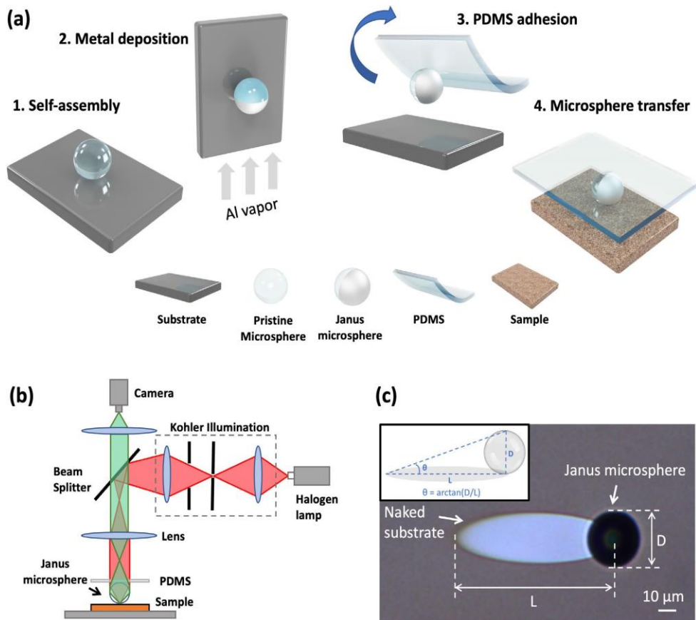
Fig. 1. (a) Illustrative drawings of the fabrication and manipulation of Janus microspheres; (b) Schematic drawing of the microsphere-assisted microscopic imaging system; (c) Optical picture of a Janus microsphere after Al deposition.
