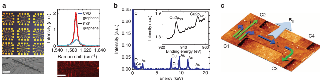
Figure 1 | Device characterization. (a) Optical image of 3 \times 3 array of devices on Si/SiO 2 substrate together with the Raman and SEM image of the active area of a typical spin Hall device. Scale bar, 5 \mu\text{m} . (b) EDX spectrum of CVDG. The samples for EDX measurements are prepared on a standard transmission electron microscopy (TEM) gold grids and are hence suspended graphene samples. The size of each grid is 7 \times 7 \mu\text{m} . The additional Au peaks in the EDX spectrum is due to the presence of Au TEM grids on which the graphene samples are prepared for analysis. Inset: XPS data on a CVD graphene sample showing the Cu 2p peaks. (c) AFM three-dimensional surface topography of a typical spin Hall device with details of actual measurement configurations.
