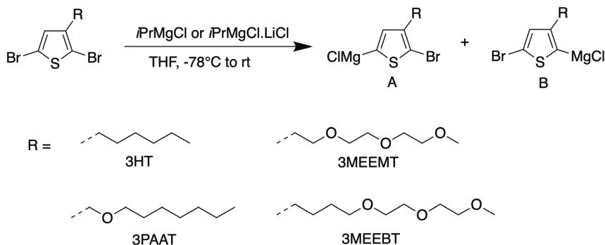
Scheme 1 Grignard metathesis of monomers 1–3.
