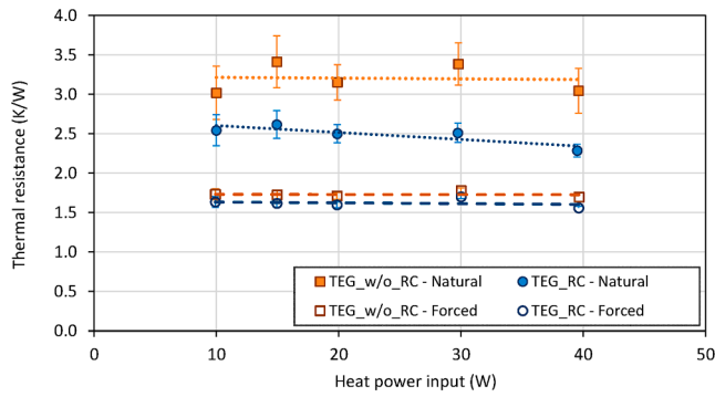
Fig. 6. Results of the thermal resistance of the heat-pipes for the TEG RC and TEG w/o RC , both under forced convection with an air velocity of 1 m/s (TEST-1) and under natural convection (TEST-2), for different heat power inputs.
