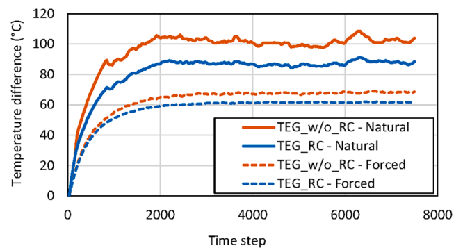
Fig. 5. Evolution of the temperature difference between the cold face of the modules and the environment of both prototypes (TEG RC and TEG w/o RC ), for 40 W of heat provided and 2.2 \Omega of load resistance.
