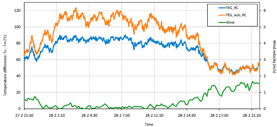
Fig. 9. Evolution of the temperature difference between the cold face of the thermoelectric modules in the generators and the environment temperature; and wind velocity over time during TEST-3.
