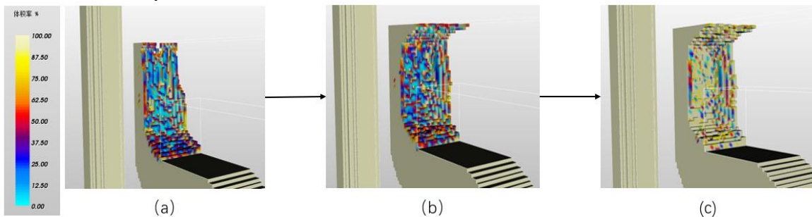
Fig. 6. Schematic diagram of volume redistribution of molten metal (a) Flow interface at the previous moment, (b) Flow interface at the next moment, before modification, (c) Flow interface at the next moment, after modification
