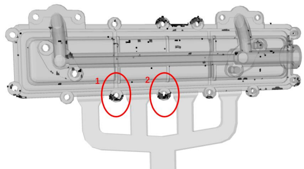
Fig. 12. Prediction results of shell entrapment defects
