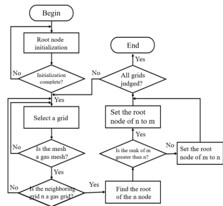
Fig. 1. Flow chart of the algorithm of the air entrainment prediction system
