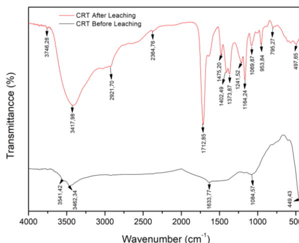
Figure 4. FTIR Spectrum of CRT Samples
