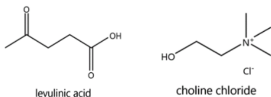
Figure 1. Structure of Levulinic Acid and Choline Chloride
