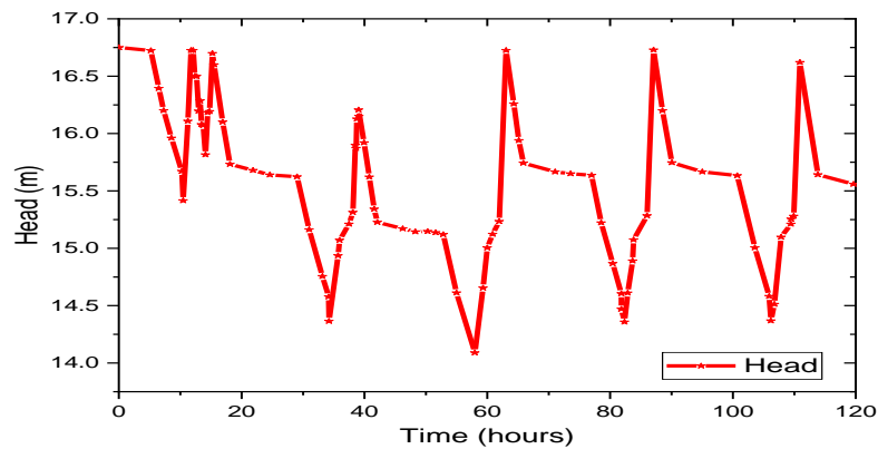
Figure 6. Storage Tank elevation change at 30 m head pump (tank no 13).
