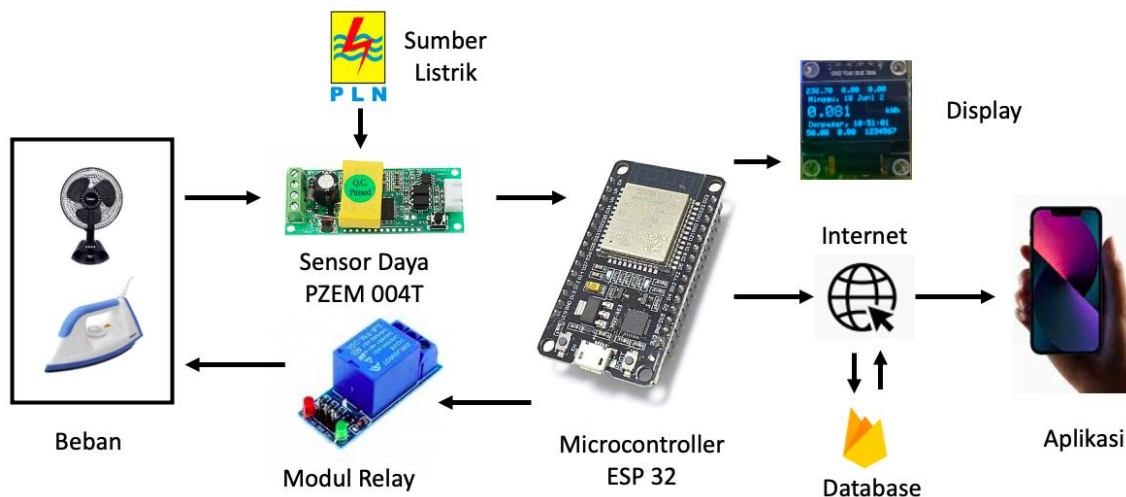
Gambar 2. Diagram Blok
