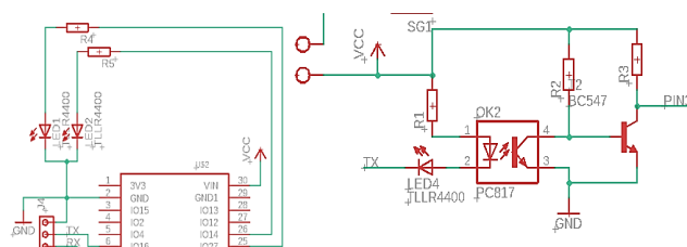
Gambar 5. Pengujian LED Indikator
