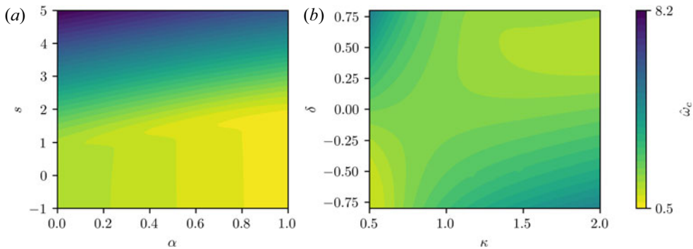
FIGURE 10. The gradient threshold as a function of equilibrium parameters. In (a) the Miller vector [\epsilon, \kappa, \delta, s_\kappa, s_\delta, \partial_r R_0, q, s, \alpha] is [1/3, 3/2, 1/2, 0, 0, 0, 2, s, \alpha] , and (b) has [1/3, \kappa, \delta, 0, 0, 0, 2, 1, 0] . In all plots \eta = 0 .
