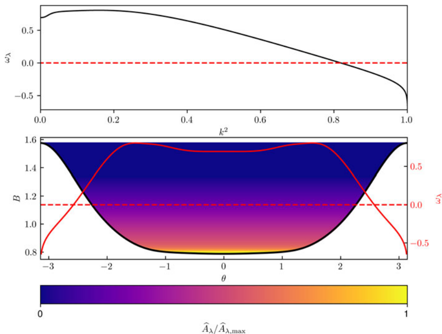
FIGURE 17. The precession frequency and \mathcal{A} distribution for a negative triangularity tokamak.
