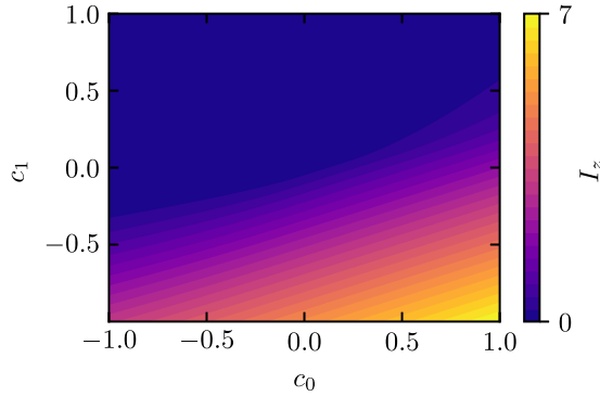
FIGURE 1. Contour plot of I_z as a function of c_0 and c_1 .
