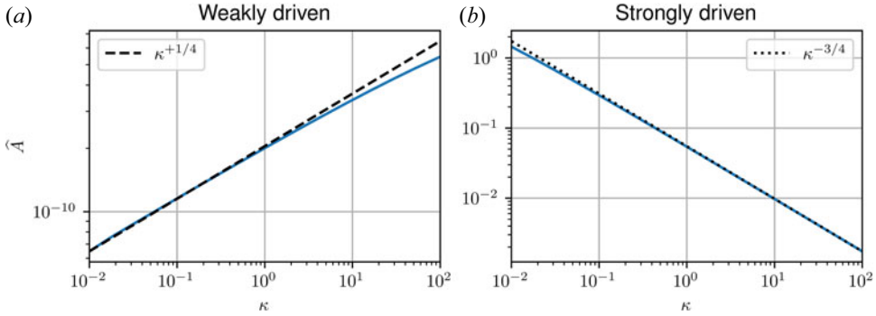
FIGURE 15. The \mathcal{A}\mathcal{E} as a function of the elongation \kappa for a very weak density gradient in (a) ( \hat{\omega}_n = 1/100 at \kappa = 1 ), and a very strong density gradient in (b) ( \hat{\omega}_n = 100 at \kappa = 1 ).
