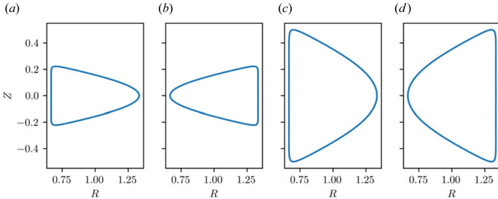
FIGURE 2. Cross-sections in the (R, Z) -plane of tokamaks parameterised via (2.53). The parameters (\kappa, \delta) vary from (a–d) as (2/3, 0.9) , (2/3, -0.9) , (3/2, 0.9) and (3/2, -0.9) , respectively. All plots have R_0 = 1 and \epsilon = 1/3 .
