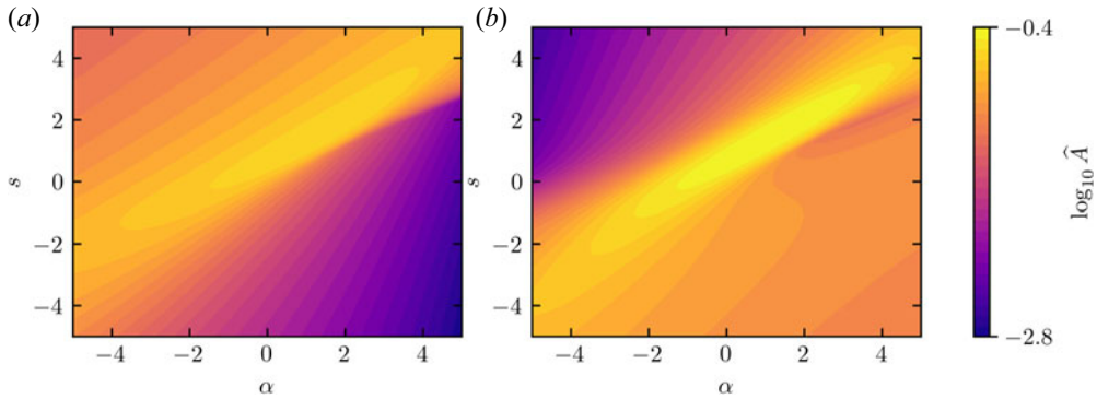
FIGURE 5. The \mathcal{A} of a large-aspect-ratio circular tokamak, as a function of magnetic shear s and pressure gradient \alpha . The plots have been generated using q = 2 . Panel (a) has \hat{\omega}_n = 3 and \eta = 0 , whereas (b) has a pure electron temperature gradient, i.e. \hat{\omega}_n = 0 and \hat{\omega}_n \cdot \eta = 3 .
