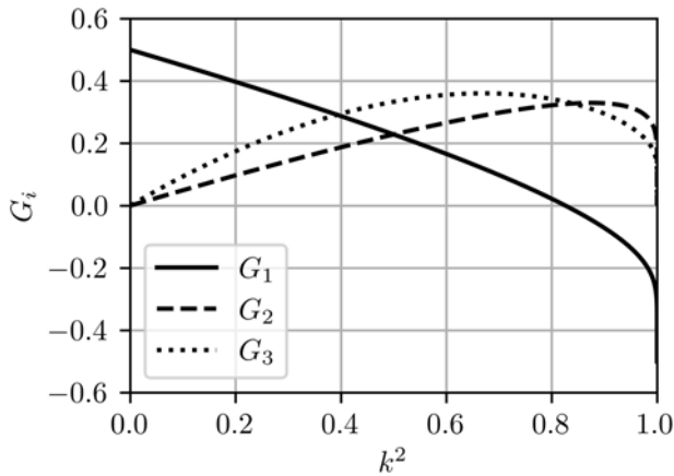
FIGURE 13. The functions G_1 , G_2 and G_3 as a function of the trapping parameter k^2 .
