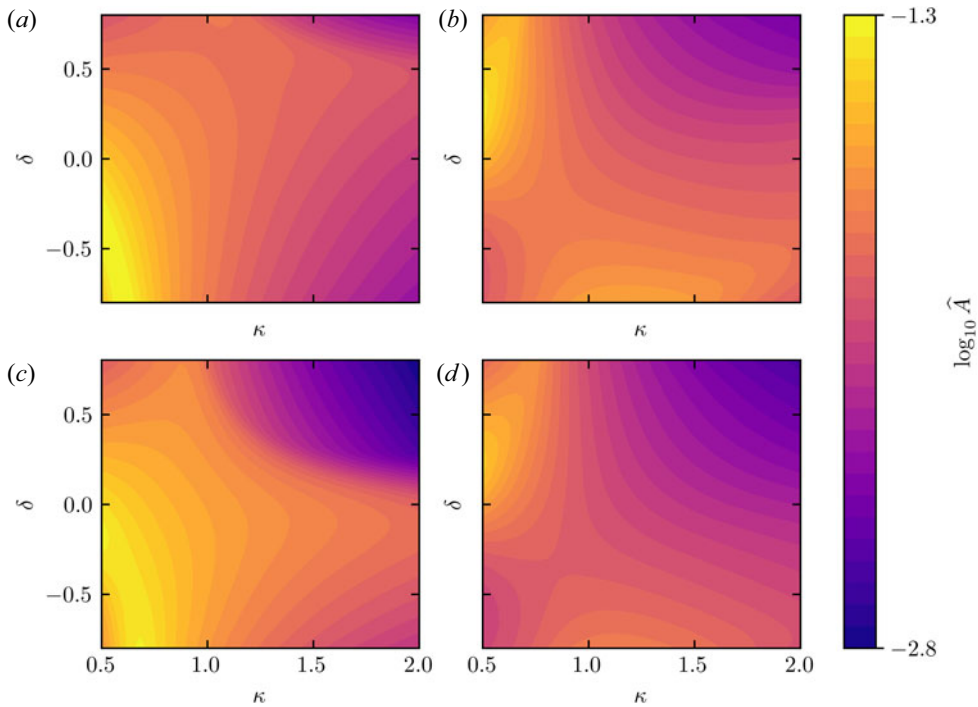
FIGURE 7. The effect of the geometry on \mathcal{A} . In (a) the Miller vector [\epsilon, \kappa, \delta, s_\kappa, s_\delta, \partial_r R_0, q, s, \alpha] is set to [1/3, \kappa, \delta, 0, 0, 0, 2, 1, 0] with \hat{\omega}_n = 1 and \eta = 0 , and all other panels have the same Miller vector with one parameter changed. The contours shown in (b) have a higher inverse aspect ratio as \epsilon is increased from 1/3 to 2/3 , in (c) the pressure gradient \alpha is increased from 0 to 1/2 , and for (d) we have decreased the shear from 1 to 0 .
