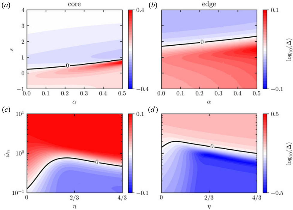
FIGURE 8. Various plots showcasing the dependencies of \log(\Delta) , where \Delta is defined as \hat{A}(\delta = -0.1)/\hat{A}(\delta = +0.1) , on various equilibrium parameters. Panels (a,c) and (b,d) have different Miller vectors [\epsilon, \kappa, \delta, s_\kappa, s_\delta, \partial_r R_0, q, s, \alpha] , which are meant to be representative of the edge and the core. Panels (a,c) have a core-like Miller vector of \mathbf{M}_{\text{core}} = [1/100, 3/2, \delta, 0, 0, 0, 1, s, \alpha] . Panels (b,d) have an edge-like Miller vector of \mathbf{M}_{\text{edge}} = [1/3, 3/2, \delta, 1/2, 0, -1/2, 3, s, \alpha] Finally, (a) has \hat{\omega}_n = 1/2 and \eta = 0 , (b) has \hat{\omega}_n = 2 and \eta = 0 , (c) has s = \alpha = 0 and (d) has s = 2 and \alpha = 1/2 .
