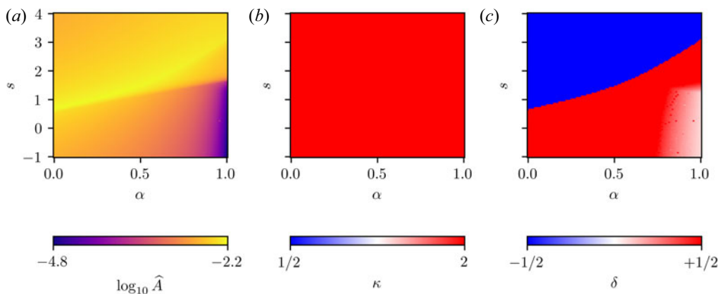
FIGURE 11. Global \mathcal{A} -minimising solutions as a function of s and \alpha . Panel (a) showcases the \mathcal{A} of the optimal solution, (b) displays the elongation and (c) shows the triangularity. Generated with a Miller vector [\epsilon, \kappa, \delta, s_\kappa, s_\delta, \partial_r R_0, q, s, \alpha] of [1/3, \kappa, \delta, 0, 0, -1/2, 3, s, \alpha] . In all panels \hat{\omega}_n = 1 and \eta = 0 .
