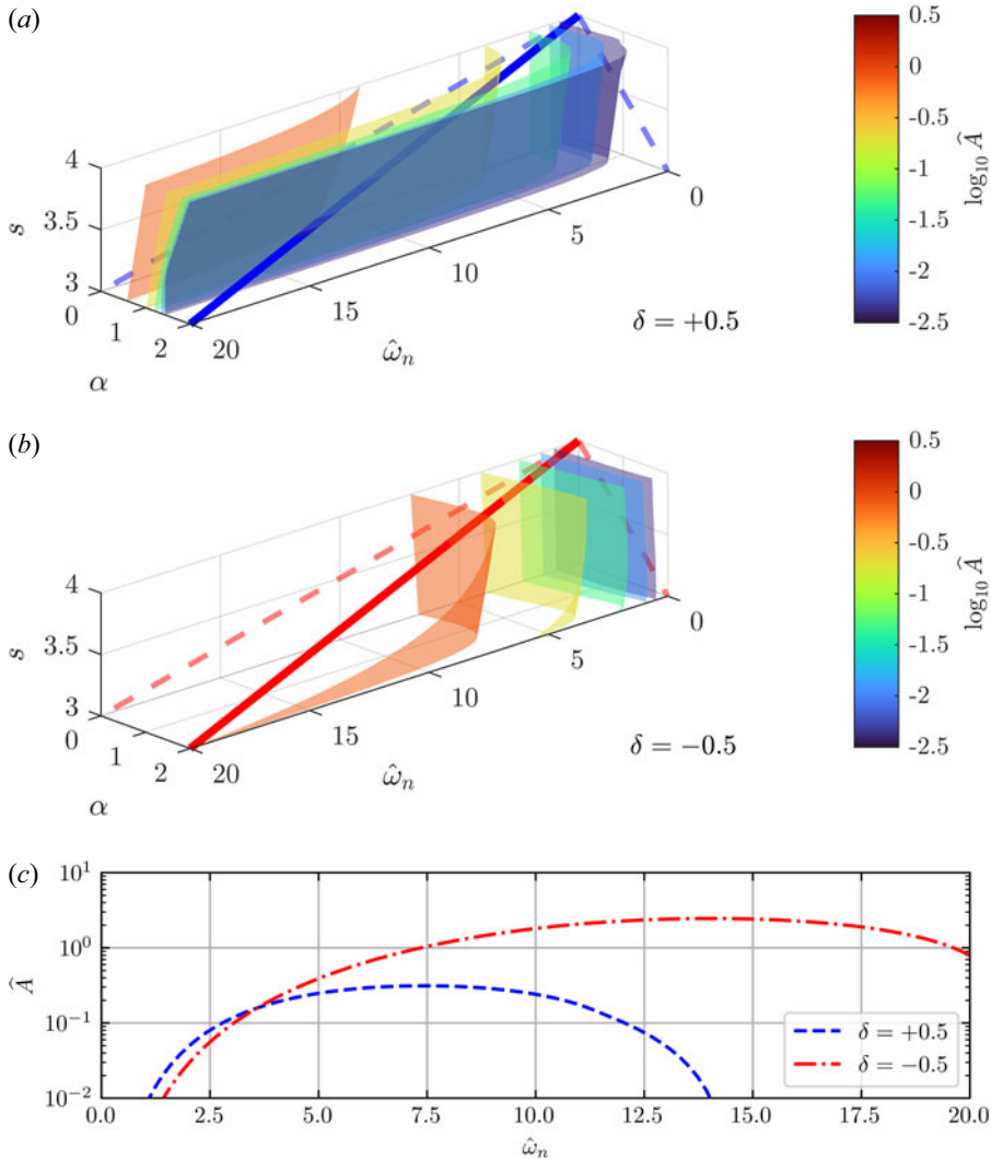
FIGURE 12. Panels (a,b) showcase isocontours of the \hat{A} as a function of (\hat{\omega}_n, \alpha, s) , where (a,b) have positive and negative triangularity, respectively. In both (a,b) a straight line is drawn which has increasing \alpha and decreasing s with increasing \hat{\omega}_n , and the projection of the line onto the grid-planes is shown as a dashed line. In (c), the \hat{A} along both the blue line of (a) and the red line of (b) is plotted as a function \hat{\omega}_n . These plots were generated with a Miller vector [\epsilon, \kappa, \delta, s_\kappa, s_\delta, \partial_r R_0, q, s, \alpha] of [1/3, 3/2, \delta, 1/2, \delta/\sqrt{1-\delta^2}, -1/2, 3, s, \alpha] , and \eta = 0 .
