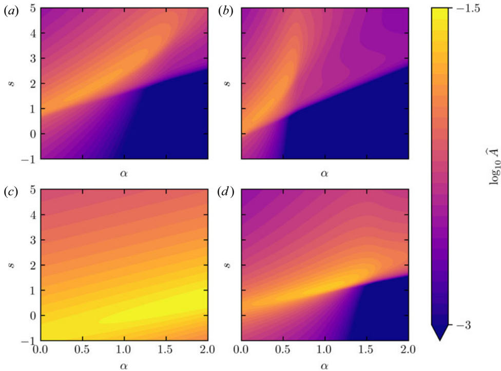
FIGURE 6. Dependence of \mathcal{A}E on magnetic shear s and pressure gradient \alpha . In (a), the Miller vector [\epsilon, \kappa, \delta, s_\kappa, s_\delta, \partial_r R_0, q, s, \alpha] is set to [1/3, 3/2, 1/2, 0, 0, 0, 2, s, \alpha] , and other panels have the same vector with one parameter changed. In (b) the safety factor q is reduced from 2 to 1, for (c) the elongation \kappa decreases from 3/2 to 1/2 , and in (d) the sign of triangularity \delta is changed from 1/2 to -1/2 . All panels have \hat{\omega}_n = 1 and \eta = 0 .
