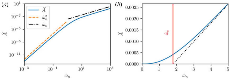
FIGURE 9. Example of dependence of \hat{\mathcal{A}} on gradient strength. Two scalings are found in (a). In (b) we define a gradient threshold by fitting a straight line to the strongly driven regime, and finding its \hat{\omega}_n interception with the abscissa.
