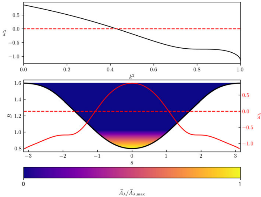
FIGURE 16. The precession frequency and \mathcal{A}E distribution for a positive triangularity tokamak.
