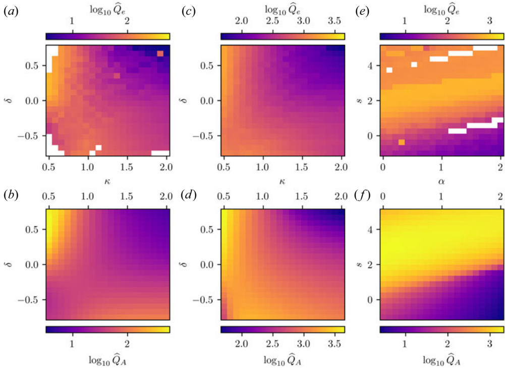
FIGURE 3. Comparison between codes, showing the correspondence between the estimate of the energy flux from \mathcal{A}\mathcal{E} and TGLF. Panels (a,c,e) display the energy flux from TGLF, and panels (b,d,f) display the corresponding estimate from \mathcal{A}\mathcal{E} . One can see agreement in trends, though some details differ. Panels (a,b) have a Miller vector [\epsilon, \kappa, \delta, s_\kappa, s_\delta, \partial_r R_0, q, s, \alpha] of [1/3, \kappa, \delta, 0, 0, 0, 2, 0, 0] , whereas panels (c,d) have [1/3, \kappa, \delta, 0, 0, 0, 2, 1, 0] , and panels (e,f) have a Miller vector of [1/3, 1, 1/2, 0, 0, 0, 2, s, \alpha] . Panels (a,b) have \hat{\omega}_n = 3 ; panels (c,d) and (e,f) have \hat{\omega}_n = 6 , and \eta = 1 in all panels. The white masked-out regions have a dominant instability which is not in the electron direction, and as such we filter them out. Finally, note that the colour bars are the same scale in each column.
