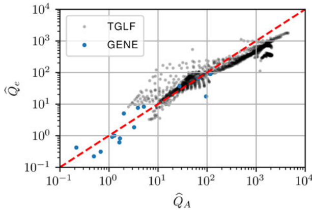
FIGURE 4. A scatter plot showing the relation between the two estimates of the nonlinear energy flux. The red dashed line shows the expected linear relationship, x = y . The plot consists of N = 1171 points. The grey points have some transparency, and as such darker regions arise due to a high density of points. Furthermore, we have added simulation data from the gyrokinetic code GENE (gyrokinetic electromagnetic numerical experiment) (Jenko, Dorland & Hammett 2001), also presented in Mackenbach et al. (2022), as blue markers.
