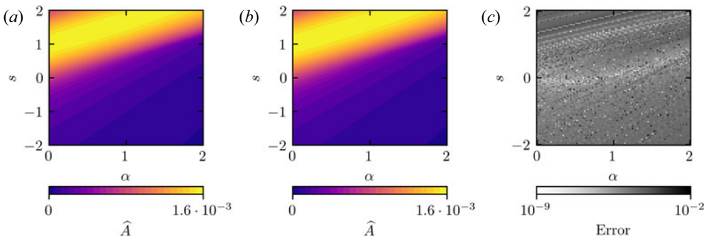
FIGURE 14. Comparison of the \bar{\mathcal{E}} as calculated with two different codes. Panel (a) is calculated using a code that calculates \bar{\mathcal{E}} in the s-\alpha limit, and (b) is calculated using the Miller code. The plots are visually indistinguishable. Calculated using q = 2 , \epsilon = 10^{-6} , \hat{\omega}_n = 3 and \eta = 1 . All other parameters for Miller are set to zero, as required in the limit of the s-\alpha tokamak. Panel (c) presents the relative error, where it can be seen that the relative error is very small for large regions of s-\alpha space. Note that the colour bar scale in (c) is logarithmic.
