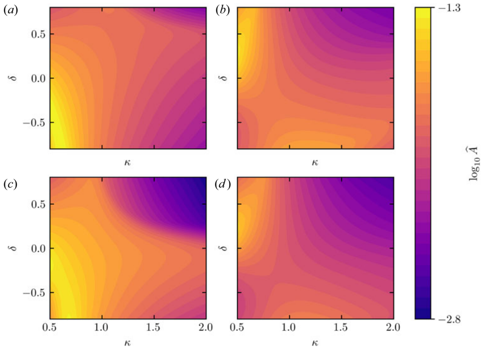
FIGURE 7. The effect of the geometry on \mathcal{A} . In (a) the Miller vector [\epsilon, \kappa, \delta, s_\kappa, s_\delta, \partial_r R_0, q, s, \alpha] is set to [1/3, \kappa, \delta, 0, 0, 0, 2, 1, 0] with \hat{\omega}_n = 1 and \eta = 0 , and all other panels have the same Miller vector with one parameter changed. The contours shown in (b) have a higher inverse aspect ratio as \epsilon is increased from 1/3 to 2/3 , in (c) the pressure gradient \alpha is increased from 0 to 1/2 , and for (d) we have decreased the shear from 1 to 0 .
