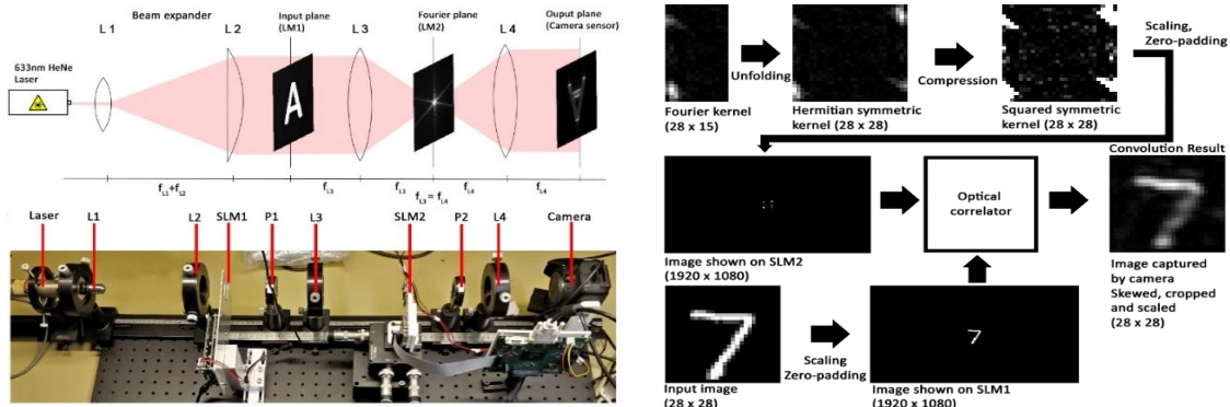
Fig. 1 – Left: The optical correlator. (Top) Schematic view of the 4F optical correlator. The character “A” is displayed as an example input image. (Bottom) Photo of the realized 4F optical correlator using off-the-shelf components. Polarizers P1 and P2 are added since liquid crystal on silicon (LCOS) SLMs are used as light modulators. Right: Procedure to perform inference on the optical correlator. All images shown in this figure are from the actual inference procedure on the optical correlator.
