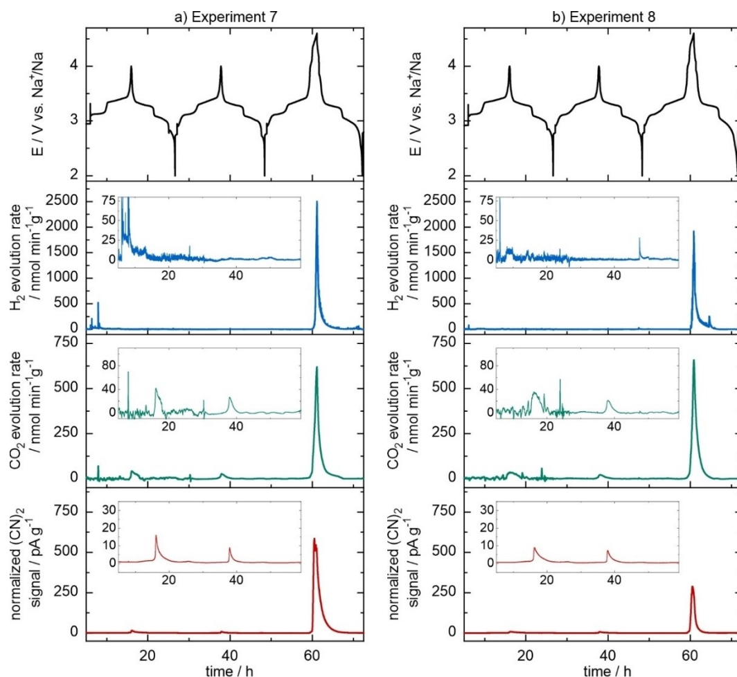
Figure 4. Gas evolution in Na half-cells with a dehydrated PW cathode using EC:PC:DMC = 1:1:1 (v/v/v) with 5% FEC as electrolyte solvent and (a) 0.3 M NaClO 4 or (b) 0.3 M NaClO 4 and 0.7 M NaPF 6 as conductive salt.
