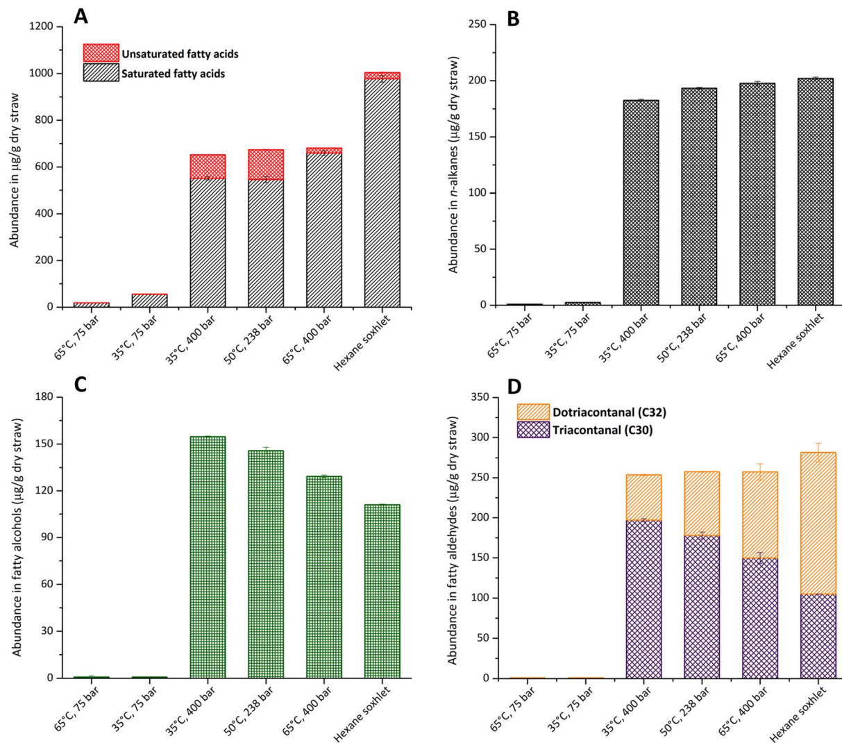
Fig. 2 Extract compositions of (A) free fatty acids, (B) n -alkanes, (C) free fatty alcohols and (D) free fatty aldehydes from rice straw waxes using \text{scCO}_2 and hexane Soxhlet extraction for 4 hours.
