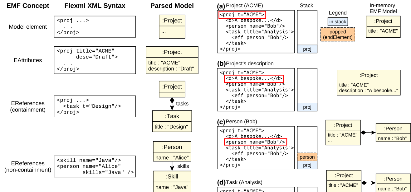
Fig. 3 XML syntax to EMF model in FLEXMI
