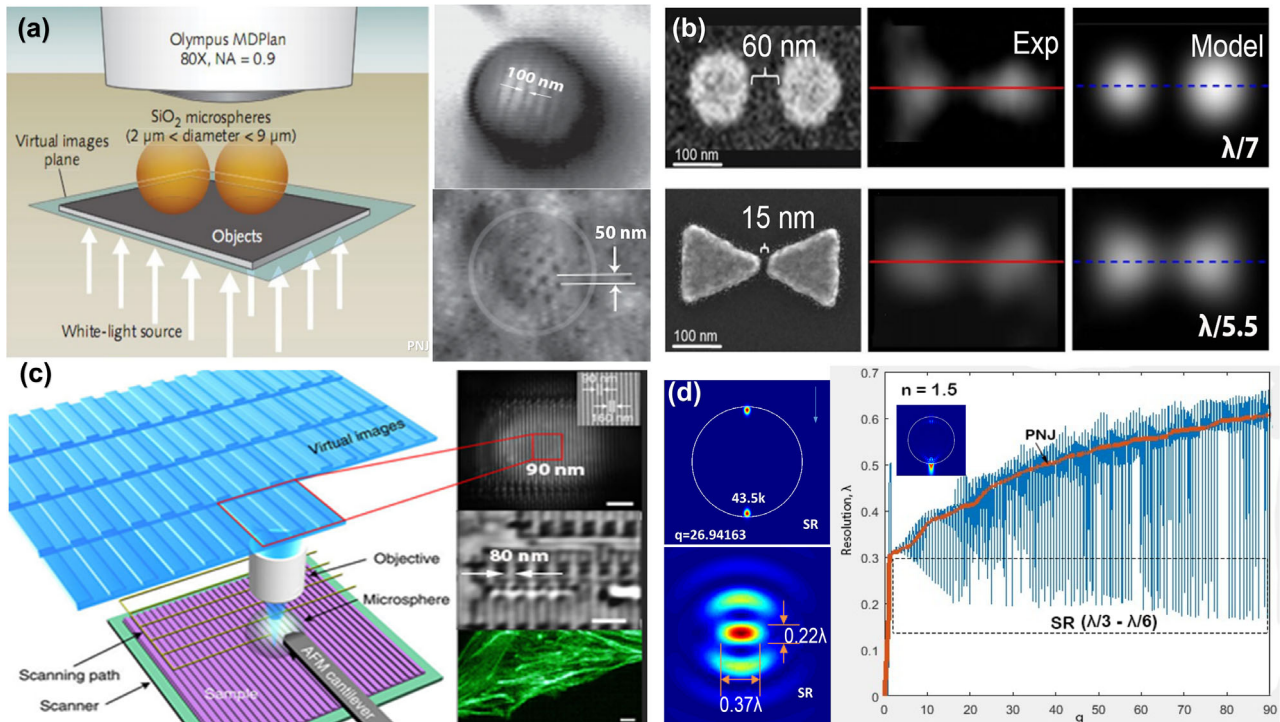
Figure 45. Microsphere nanoscopy. a) Contact mode setup and imaging examples (50–100 nm samples). Reproduced with permission. [136] Copyright 2011, Wiley-VCH. b) Resolution analysis by the PSF convolution method ( \lambda = 405 , confocal mode). Reproduced with permission. [138] Copyright 2015, Wiley-VCH. c) Non-contact scanning superlens imaging setup and examples (microsphere attached to AFM tip, sample: 80–90 nm nanodevices, and fluorescent-labeled actin filament). Reproduced with permission. [612] Copyright 2016, Springer Nature. d) SR mode demo at size parameter q = 26.94164 with peak value \approx 43.5k and theoretical resolution \approx \lambda/3 - \lambda/6 for n = 1.5 , q = 0-90 microspheres.
