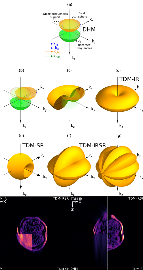
Figure 22. Optical Transfer Function (OTF) for various configurations in transmission TDM. a) Digital holographic microscopy: the OTF depicts a cap of sphere with large lateral, but limited longitudinal extension. b) With inclined illumination, same positions of \mathbf{k}_{diff} vectors provide new \mathbf{k}_{obj} vectors. c, d) With many illuminations, a filled, extended OTF is obtained. e) With sample-rotation, an almost completely filled sphere is obtained (but of lesser extension than in previous case). f, g) OTFs combining illumination and sample rotation with 2, and 4 evenly spaced specimen positions. Bottom row: Betula pendula pollen grain images in DHM and three TDM variants. Left composite image depicts x-y slice in the focal plane, showing improved resolution in TDM, but only twice that of DHM. Contrast is however better thanks to better optical sectioning. Right composite image highlights the large differences in imaging capabilities along the optical axis. Only TDM-IRSR can deliver true improved and isotropic resolution, while holography is not, strictly speaking, a true 3-D imaging method when considering transparent samples: only optical thickness can be measured.
