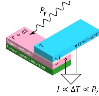
Figure 2. Schematic idea for biasless detection based on thermoelectricity. Absorbed light with power P_\gamma heats up one part of the heterostructure, creating a temperature difference \Delta T , which results in a thermoelectric current I = \alpha \Delta T / T \propto P_\gamma .
