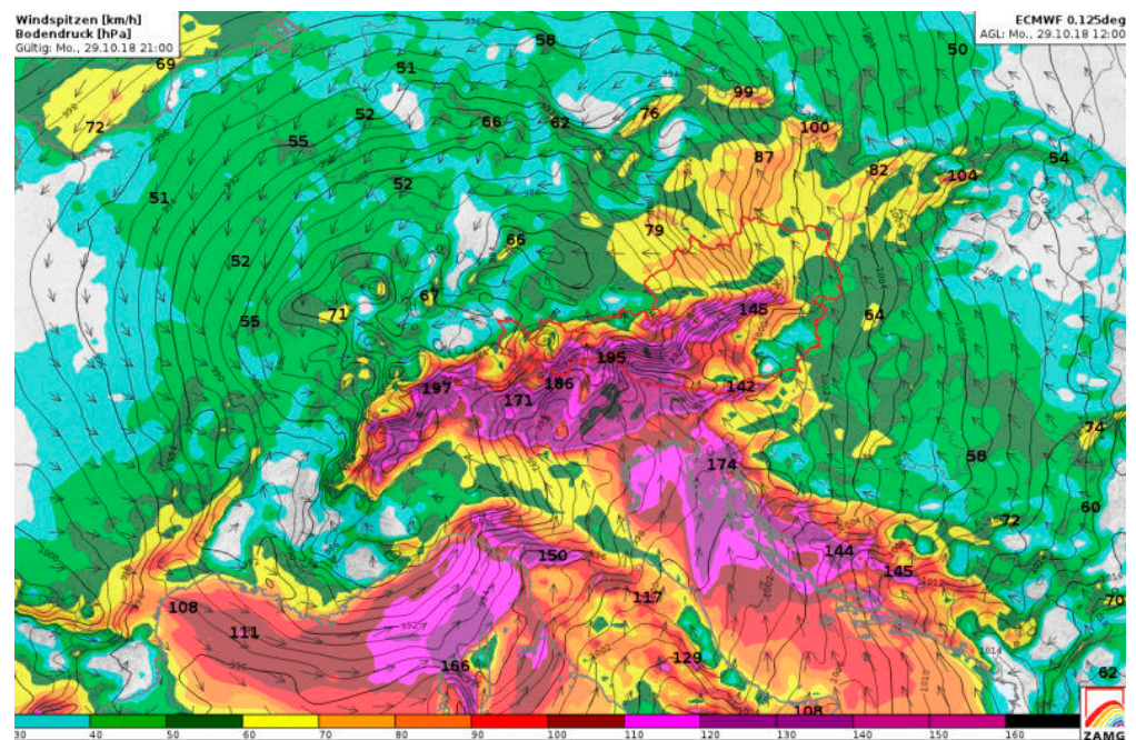
Figure 2. Synoptic chart for storm Vaia on 29 October 2018 (ECMWF, European Centre for Medium-Range Weather Forecasts).
