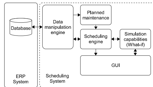
Fig. 2. Design characteristics for a production scheduling system.
